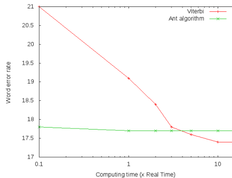
Fig. 3. Comparison between Viterbi beam-search and ant colonies algorithm: Computing time against performance, on the dev set with a 4-gram language model. With time constraints the ant algorithm is more efficient than a conventional extension.
