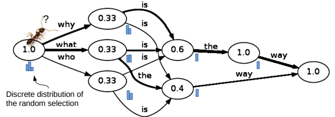
Fig. 1. In order to leave a node, ants will have to choose a link. This choice is performed with a weighted random selection based on the quantity of pheromone on each arc (weighted by the nodes posteriors in our experiments). The thickness of the line expresses the amount of pheromone already deposited.
