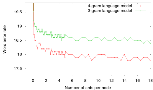
Fig. 2. Evolution of rescoring according to the number of ant by node (on the dev set) during 1 run.
