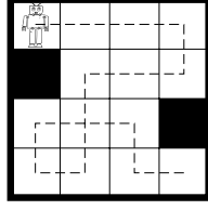
Figure 2 – \iota\sigma_B^P(G_{4,4}) \leq 2 .
