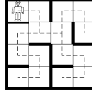
Figure 3 – \iota\sigma_W^S(G_{4,4}) \leq 9 .
