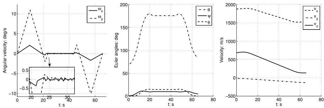
Figure 12: State variable x(t) ( v_0 = 2000 m/s).
