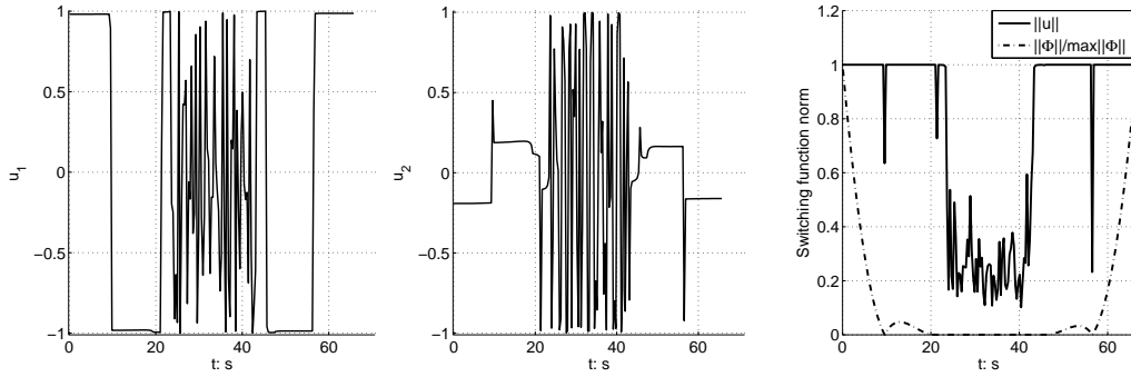
Figure 13: Optimal control and \|\Phi(t)\| ( v_0 = 2000 \text{ m/s} ).
