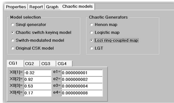
Fig. 22. Selection chaotic generator, model and initial conditions in the software to signal analysis
