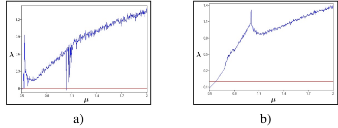
Fig. 5. Function of the Lyapunov exponent for 2-D new maps a) TTL_{\mu}^{RC} non-alternate map (10) b) TTL_{\mu}^{SC} alternate map (11)
