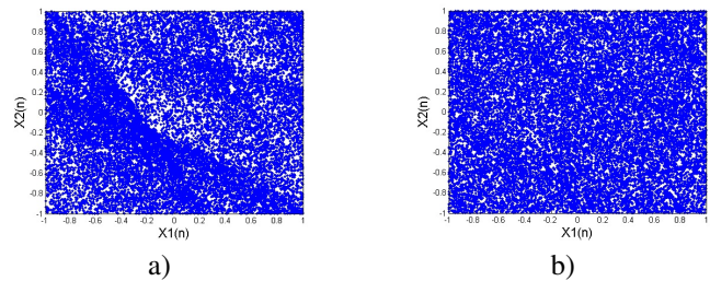
Fig. 6. Phase space attractor of 2-D new maps, 2 \times 10^4 points are generated a) TTL_{\mu}^{RC} non-alternate (10) b) TTL_{\mu}^{SC} alternate (11)
