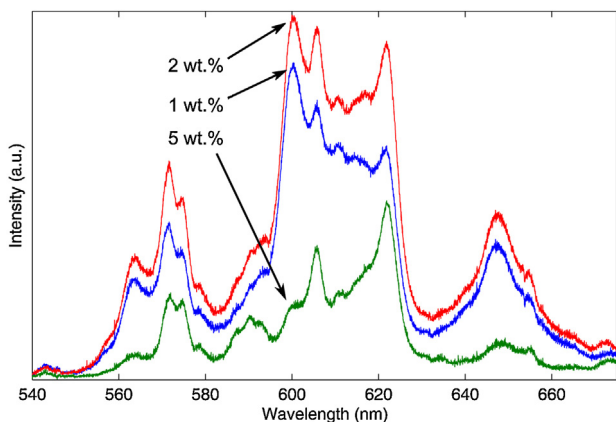
Fig. 6. The phosphorescence emission spectra from YSZ:Sm powder samples with three different dopant concentrations.
