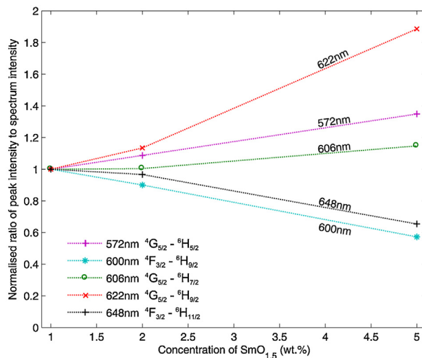
Fig. 7. The relative change in the intensity at the emission peaks as the dopant concentration increases is shown by plotting the ratio of the integrated intensity at each emission peak (1 nm bandwidth) to the integrated intensity of the full recorded spectrum (560–670 nm). The values are normalised at the value for 1 wt.% SmO_{1.5} to depict the trends.
