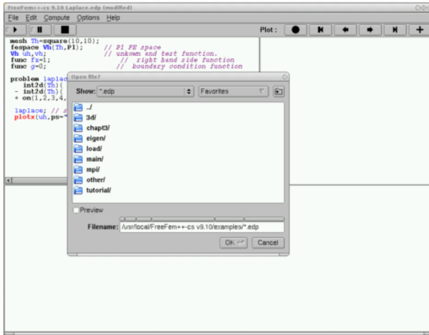
Figure 5: File/Open Example...
