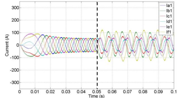
Fig. 12: H-bridge's current with reconfiguration 2.
