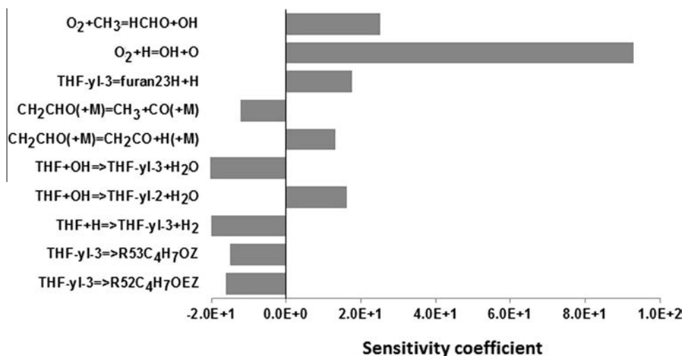
Fig. 17. Sensitivity analysis on \text{OH}^* radicals for ignition delay time at \phi = 1.0 (1% THF/5.5% \text{O}_2 /93.5% Ar), 1423 K, and 8.58 atm.
