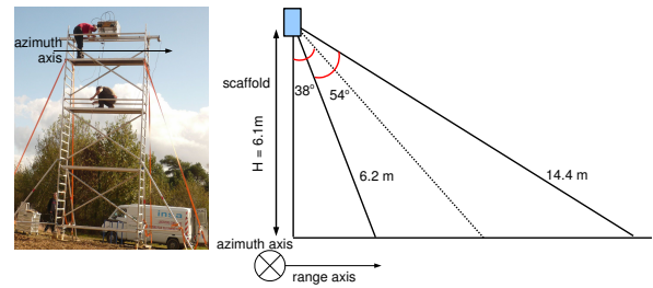
Fig. 1. Geometric configuration of the GB-SAR campaign.
