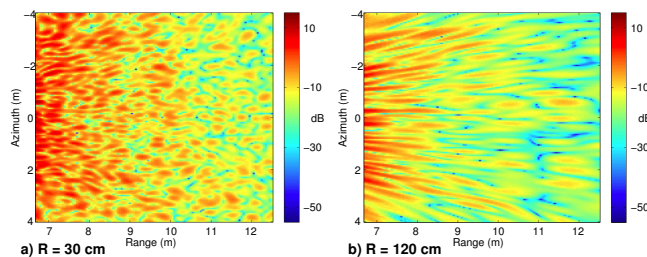
Fig. 4 The processed and calibrated GB-SAR backscattering coefficients (HH polarization) at different resolutions of R .
