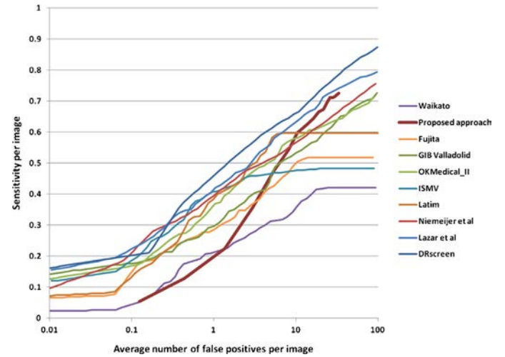
Fig. 15. FROC curves of the ROC methods.
