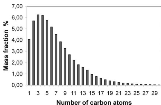
Fig. 6. Mass distribution of n -alkanes used to model the first six compositions of Table 3.
