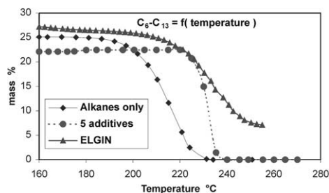
Fig. 8. Evolution of the mass fraction of the n\text{-C}_6 to n\text{-C}_{13} fraction of mixtures 1, 6 and 7 of Table 3, subjected to a heating rate of 1.5\text{ °C par Ma} .
