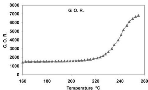
Fig. 10. Evolution of the gas to oil ratio of ELGIN oil subjected to a heating rate of 1.5\text{ °C per Ma} .
