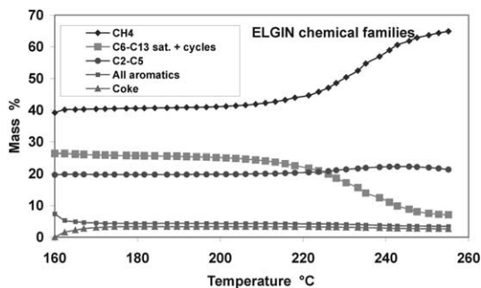
Fig. 9. Evolution of the distribution of chemical families during the heating of ELGIN oil (composition 7 of Table 3), at a rate of 1.5\text{ °C par Ma} .
