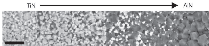
Fig. 5. Illustration of the junction between AlN and TiN, with a concentration gradient. Backscattered electrons SEM-FEG images show AlN-phase (dark) and TiN-phase (bright) (Bar= 10 μm).
