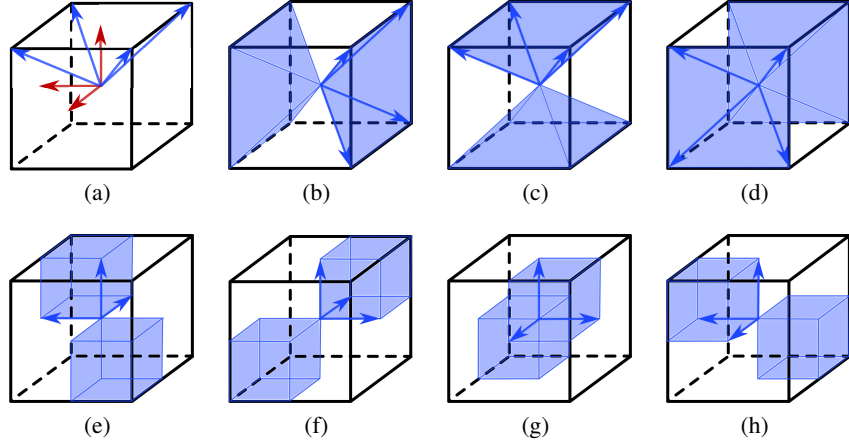
Fig. 2. (a) The 7 orientation vectors of \mathcal{D} (principal orientations in red, principal diagonals in blue). The cones of orientations associated to the red vectors (b–d) and to the blue vectors (e–h).
