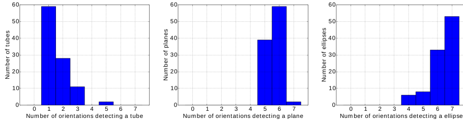
Fig. 3. Ratio of path opening high responses, computed from 100 binary synthetic examples: (left) a tube, (center) a plane, and (right) a curved plane, within the set \mathcal{D} of 7 orientations illustrated in Figure 2.
