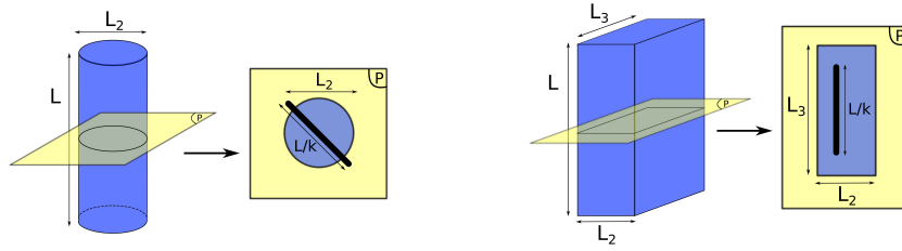
Fig. 1. A segment SE (in black) of length L/k cannot fit a 1D object (left) but can fit a 2D one (right), in the plane P orthogonal to the orientation of their largest dimension (see text).
