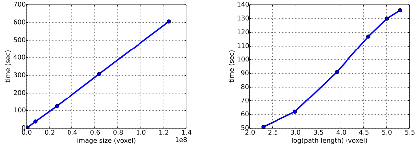
Fig. 4. Computational cost of RORPO, with respect to |\mathcal{Q}| (left) and L (right, log scale).
