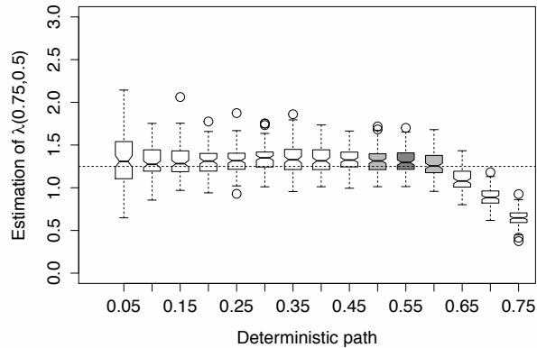
Figure 7: The estimator \hat{\lambda}_\xi^n(x) is computed from different values of the index \xi \in \mathcal{C}_x , and from the optimal bandwidth parameters obtained at Steps 1 and 3. Over the 100 replicates, the optimal points \hat{\xi}_*^n obtained at Step 2 are most of the time located at 0.55 and more than 90 times between 0.5 and 0.6 (enhanced by gray colors), which seems to correspond with the estimators with least bias and variance. In particular, we obtain a better result than by maximizing the estimated invariant measure \hat{\nu}_\infty^n (index around 0.35), see Remark 3.11.
