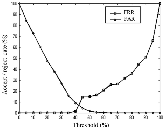
Fig. 10 False rejection and acceptance rates against threshold of hand shape modality.
