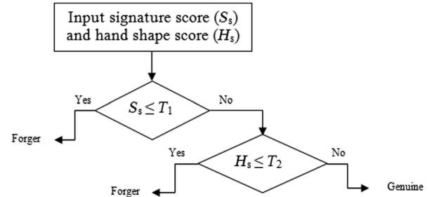
Fig. 11 Adopted decision tree.
