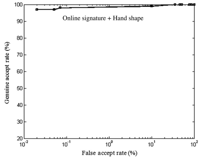
Fig. 15 ROC curve showing an improvement in performance by combining signature and hand shape modalities.
