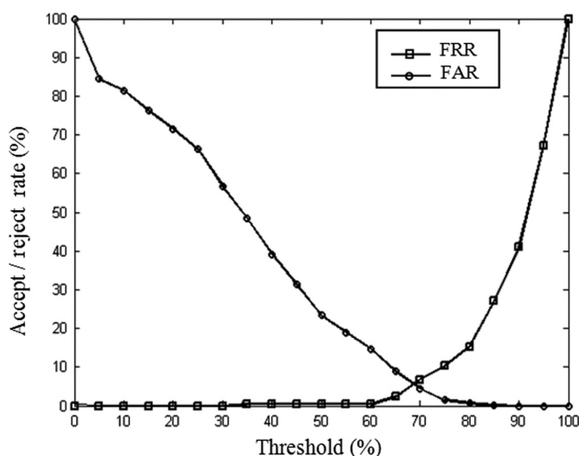
Fig. 5 False rejection and acceptance rates against the threshold of online signature modality.
