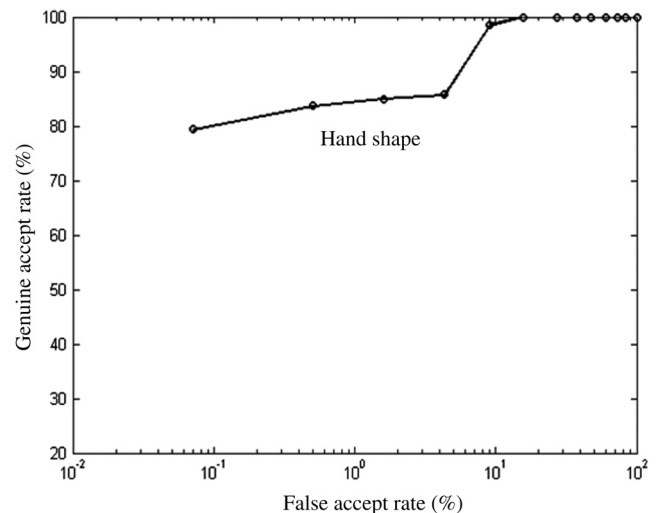
Fig. 9 ROC curve showing the performance of hand shape modality.
