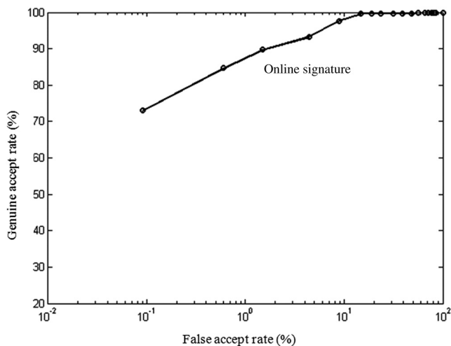
Fig. 4 ROC curve showing the performance of online signature modality.
