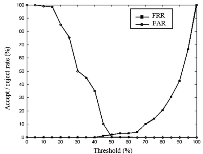
Fig. 16 False rejection and acceptance rates against threshold of combined signature and hand shape modalities.
