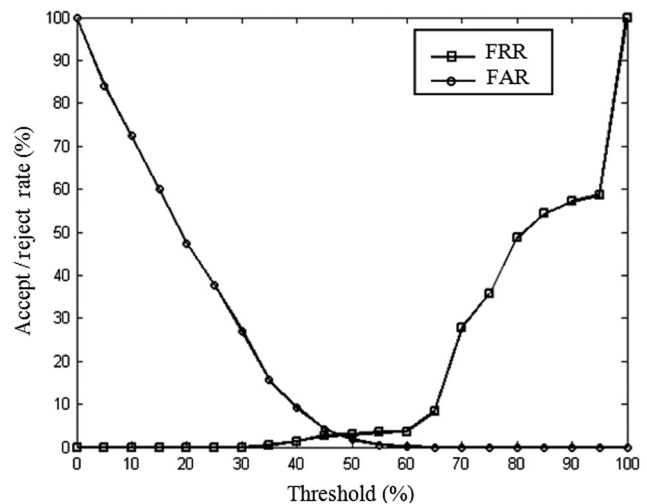
Fig. 13 False rejection and acceptance rates against threshold of combined signature and hand shape modalities.
