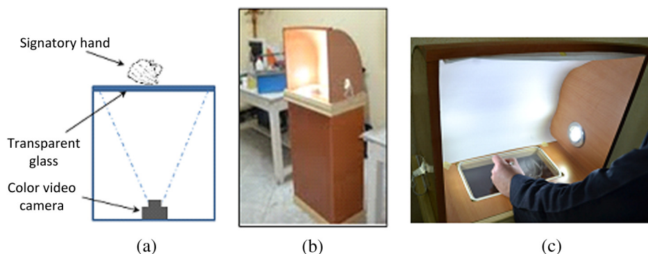
Fig. 1 Used online signature acquisition system: (a) global view, (b) laboratory prototype, and (c) signing operation view.
