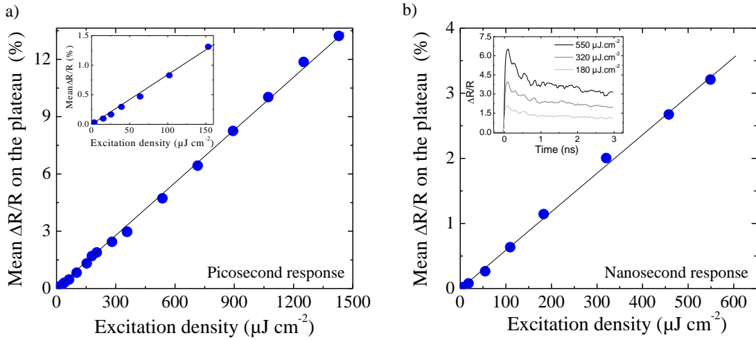
FIG. 9. (Color online) Plateau signal for 1.46 eV pump and 1.72 eV probe, integrated between 6.5 and 8.5 ps at 100 K (a). The blow up of the excitation densities under 150 \mu\text{J}\cdot\text{cm}^{-2} is in the inset. Plateau signal integrated between 2.3 and 3 ns (b). The inset shows the photoresponse at different excitation densities.
