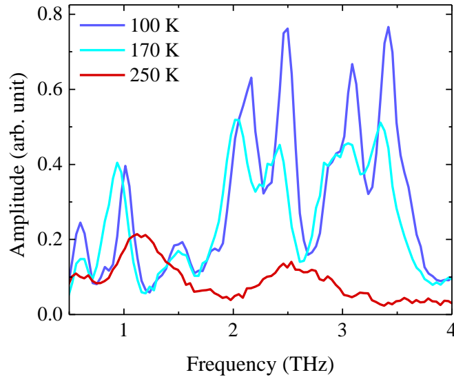
FIG. 4. (Color online) Raman spectra of (\text{EDO-TTF})_2\text{SbF}_6 in the I phase at 100 K and 170 K and in the M phase at 250 K.
