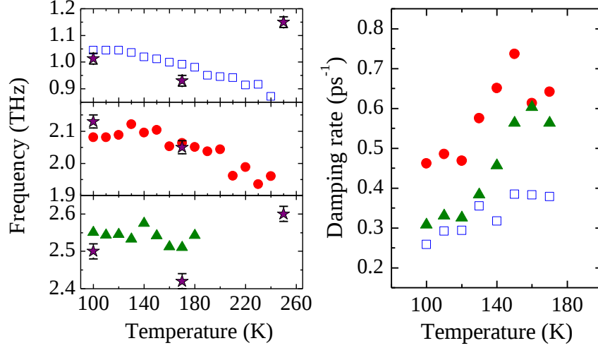
FIG. 10. (Color online) (a) Temperature dependence of frequencies for the 3 main modes at around 1 THz (□), 2 THz (●) and 2.5 THz (▲) from the fit model and by Raman spectroscopy (★) from 100 K to 240 K. (b) Temperature dependence of damping rate.
