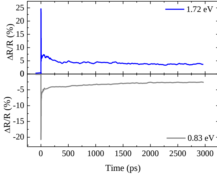
FIG. 5. (Color online) Photoresponse of (EDO-TTF) 2 SbF 6 at 100 K for a 1.46 eV pump and 1.72 eV probe (upper graph) and 0.83 eV probe (lower graph).
