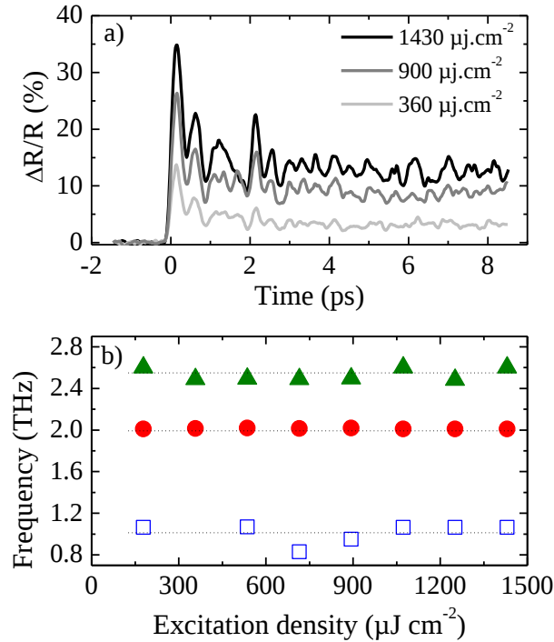
FIG. 8. (Color online) (a) Photoresponse of (\text{EDO-TTF})_2\text{SbF}_6 at 100 K for 1.46 eV pump and 1.72 eV probe at different fluencies. (b) Photon excitation density dependence of the phonon frequencies at 100 K.
