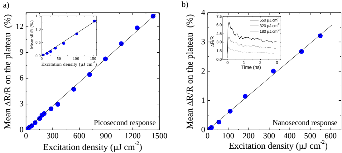
FIG. 9. (Color online) Plateau signal for 1.46 eV pump and 1.72 eV probe, integrated between 6.5 and 8.5 ps at 100 K (a). The blow up of the excitation densities under 150 \mu\text{J}.\text{cm}^{-2} is in the inset. Plateau signal integrated between 2.3 and 3 ns (b). The inset shows the photoresponse at different excitation densities.
