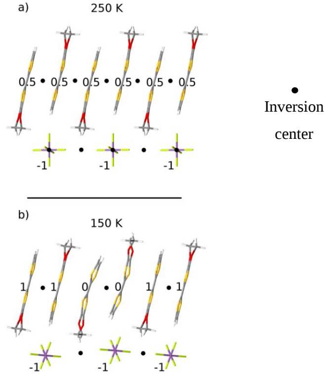
FIG. 1. (Color online) Crystal structures of the M (a) and I phase (b) and the corresponding schematic charge distribution on the D molecules. In the I phase, the symmetry breaking resulting from charge ordering involves important structural reorganization with, for example, the bending of the neutral molecules. Due to the cell doubling along the stack, the inversion symmetry is lowered, and the charge ordering accompanied by important modifications of the orientation of the \text{SbF}_6^- anions is observed.
