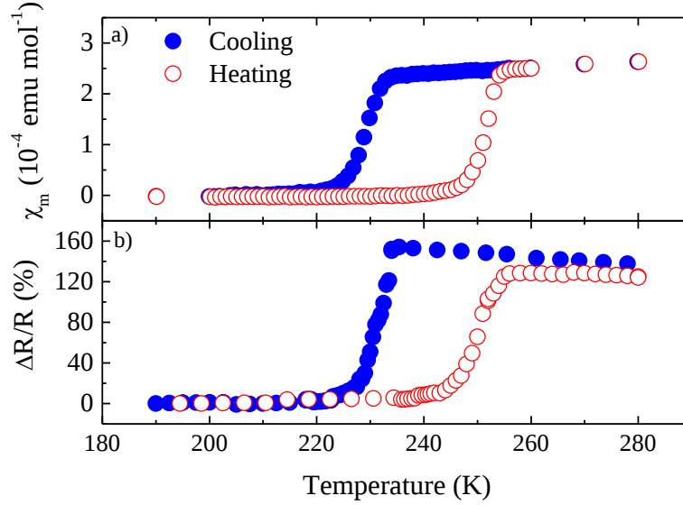
FIG. 2. (Color online) (a) Magnetic susceptibility of (\text{EDO-TTF})_2\text{SbF}_6 and (b) relative variation of the reflectivity at 1.72 eV as a function of temperature with a polarisation parallel to the D chain cell parameter b of (\text{EDO-TTF})_2\text{SbF}_6 : the hysteresis is centred at 240 K and 22 K wide.
