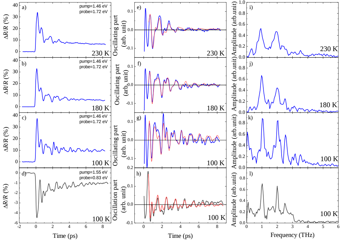
FIG. 6. (Color online) Photoresponse of (\text{EDO-TTF})_2\text{SbF}_6 at 100 K, 180 K and 230 K for a 1.46 eV pump and 1.72 eV probe (a-c) and a 1.55 eV pump and 0.83 eV probe (d). Oscillation part retrieved from the photoresponse and the corresponding fit (thin red – or light gray- lines) with 3 phonon modes (e-h correspond to a-d, respectively). The transformed Fourier spectra obtained from the oscillation (i-l correspond to e-h, respectively).
