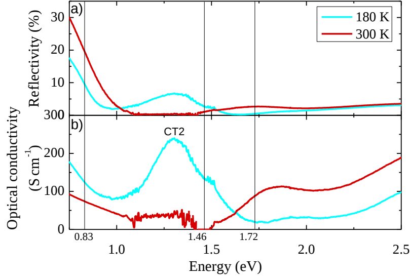
FIG. 3. (Color online) (a) Reflectivity R at different temperatures with a polarisation parallel to the D stacking axis of (EDO-TTF)_2SbF_6 . (b) Optical conductivity of (EDO-TTF)_2SbF_6 .
