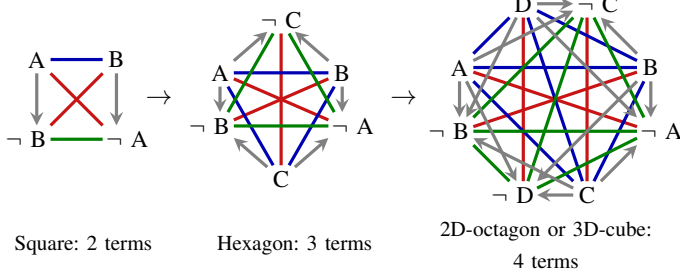
Figure 5. n -partition polygons maintaining the 4 relations of the classical square [18]
