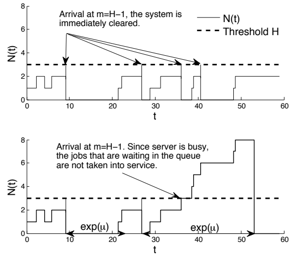
Fig. 1: Simulation of process N(t) , number of waiting jobs at time t , under threshold H = 3 . Above the \mu = \infty case, below the \mu < \infty case. Below exp(\mu) refers to the busy period of the server, which is exponentially distributed with rate \mu < \infty . As a consequence N(t) not only depends on H but also on the length of each busy period.
