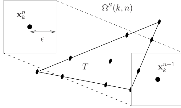
Figure 1: Example of a triangular mesh cell T (with its Fekete points for q = 3 ) intersecting the convex support \Omega^S(k,n) of the k -th particle moving on the time step [t_n, t_{n+1}] .
