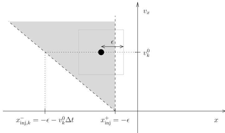
Figure 3: Phase-space profile of the smooth particle injection. For a charge-conserving injection, particles must be loaded at each time step in a “virtual” region (outside the computational domain x \geq 0 ) where the inflow distribution f_{\text{inj}} is extended uniformly with respect to x < 0 . For an accurate discretization with smooth shapes of radius \epsilon , particles with an initial speed of v_x = v_k^0 must then be loaded following this virtually extended distribution on an interval [-\epsilon - v_k^0\Delta t, -\epsilon] .
