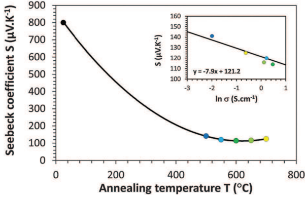
Fig. 6 The measured Seebeck coefficients ( S ) for 100 nm thick films annealed at different temperatures. Inset: Jonker's plot.
