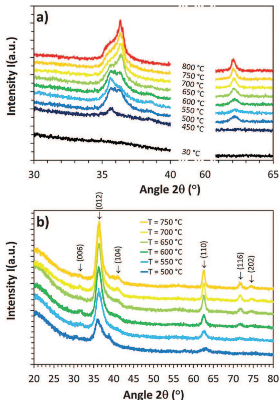
Fig. 2 XRD patterns of 300 nm thick Mg-doped \text{CuCrO}_2 films. (a) In situ TXRD patterns registered in \theta – \theta Bragg–Brentano geometry at various temperatures in the range of 30 to 800 °C under primary vacuum and (b) \alpha = 1^\circ GIXRD patterns registered at room temperature after similar ex situ annealing treatment.
