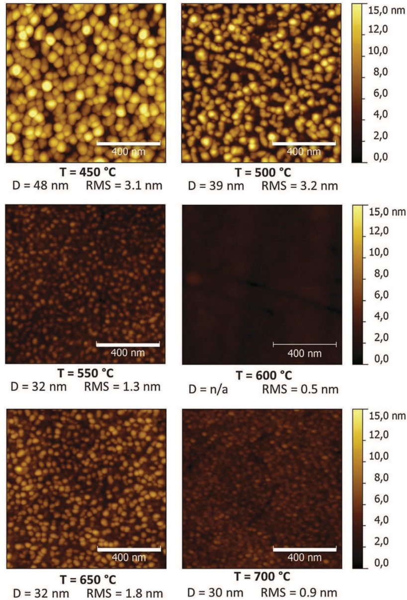
Fig. 4 AFM micrographs of 100 nm Mg-doped \text{CuCr}_2 annealed at various temperatures in the range of 450 °C to 700 °C for 4 h under primary vacuum. The average particle size ( D ) and root mean square roughness (RMS) are indicated for all the samples.
