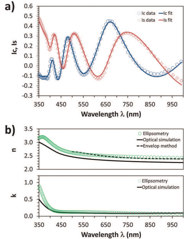
Fig. 8 300 nm thick Mg-doped \text{CuCrO}_2 film annealed at 600 °C optical constants. (a) Experimental and simulated ellipsometric data I_s ( \sin 2\Psi \times \sin \Delta ) and I_c ( \sin 2\Psi \times \cos \Delta ) as a function of optical wavelength, and (b) the corresponding optical constants, n and k , determined from analysis of ellipsometry data (green circles), and TT and TR data (refinement of the dielectric model is indicated by the black full line and the envelop method is indicated by the dashed line).
