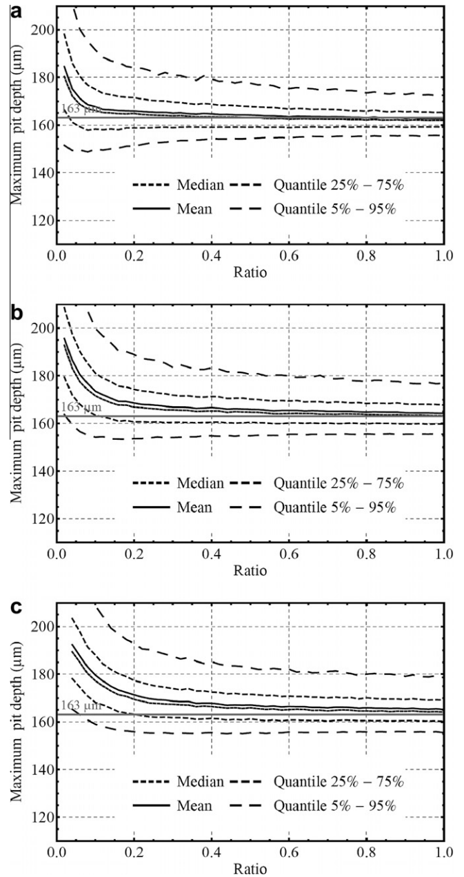
Fig. 9. Evolution of the maximum pit depth realizations on the whole sample as a function of the area ratio for the mean, the median, the 5th, 25th, 75th and 95th quantiles considering the Gumbel approach. The selected area has been divided into 5 (a), 10 (b) and 15 (c) samples in order to estimate parameters \mu and \sigma .
