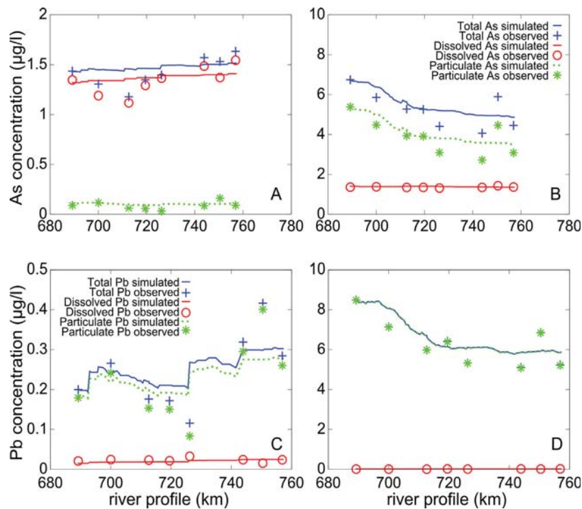
Fig. 7. Simulations of arsenic (A, B) and lead (C, D) concentrations during low-water flows (A and C, respectively, flow of 80\ m^3\ s^{-1} , continuous line) and high-water flows (B and D, respectively, flow of 800\ m^3\ s^{-1} , continuous line). The dissolved and particulate phases are shown with the total concentration in the water. Observation results were indicated for the different fractions and hydrological conditions using corresponding symbols. Note the different concentration scale for the two hydrological conditions.
