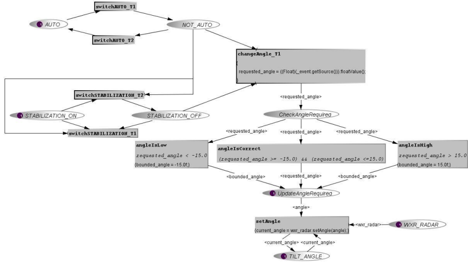
Fig. 5. Cooperative Object (CO) model of the weather radar control panel
