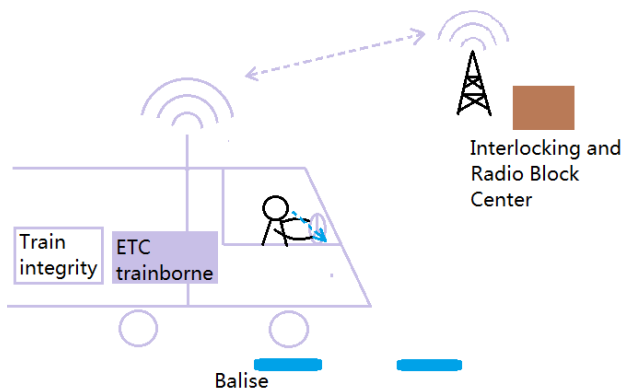
Figure 3: ERTMS/ETCS Level 3
