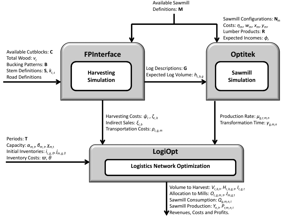
Figure 4: Interactions between FPInterface–Optitek and LogiOpt.
