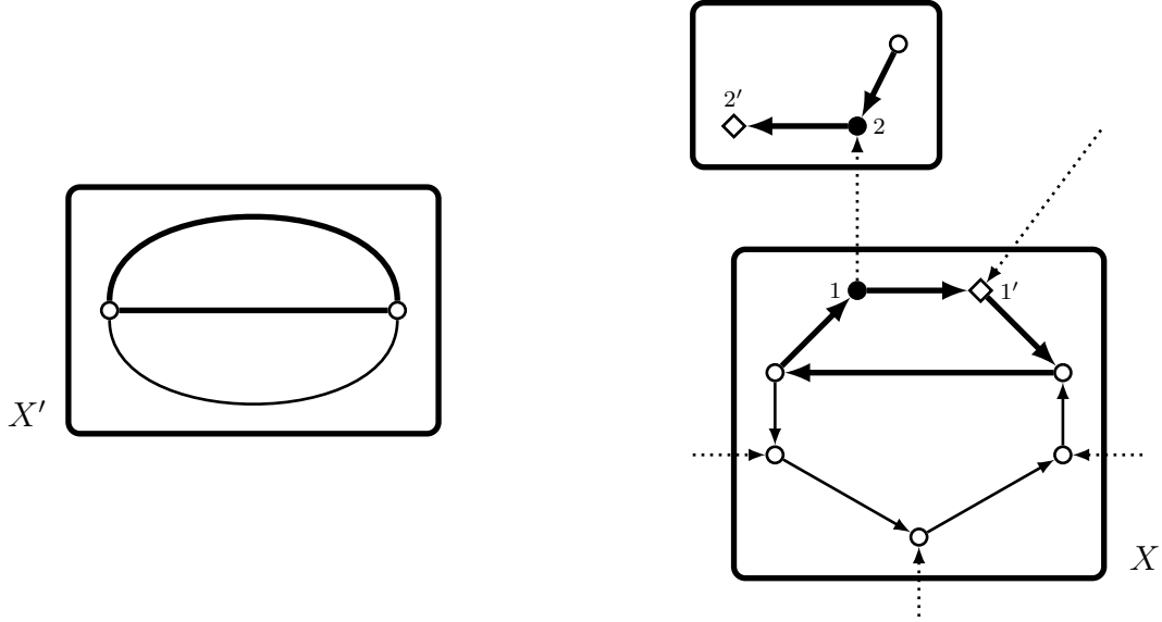
Figure 9: An example of how the orientation \vec{G} is obtained, and an application of the firefighting strategy on \vec{G} , as described in the proof of Theorem 5.5. Thin arcs (respectively, edges) represent path arcs (respectively, edges in the perfect matching P' ), the thick arcs (respectively, edges) represent cycle arcs (respectively, edges in the 2-factor C' ), and the dotted arcs represent bridge arcs.
