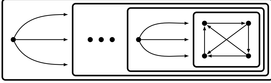
Figure 7: The orientation of a 3-tree described in the proof of Proposition 5.3.
