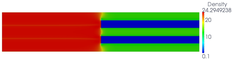
Figure 24: Test case B. Density distribution around the steady state for mesh 5 in region [0, 5] \times [0, 1] .
