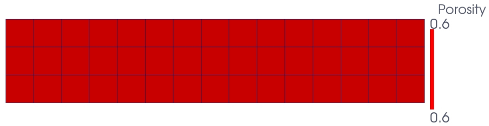
Figure 4: Test case A. Porosity distribution for mesh 2 including 15 \times 3 cells.
