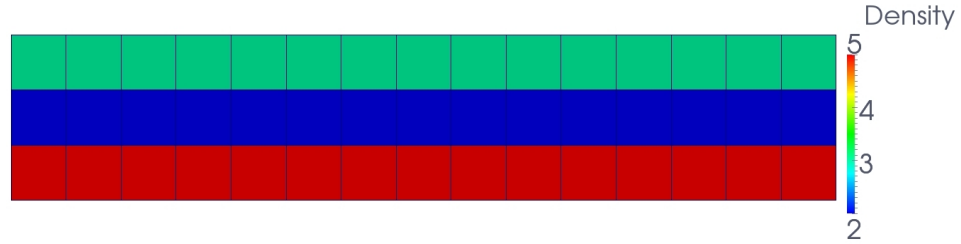
Figure 7: Test case A. Density distribution for mesh 2 including 15 \times 3 cells.
