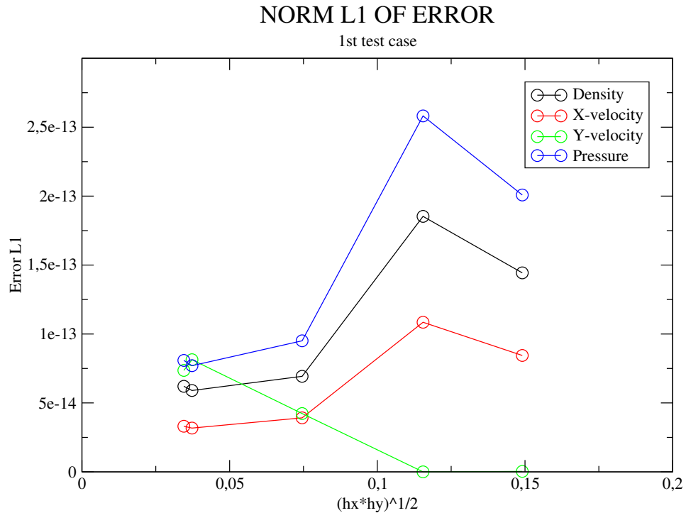
Figure 9: Test case A. L^1 norm of the error versus mesh size h , for the density, velocity and pressure variables.
