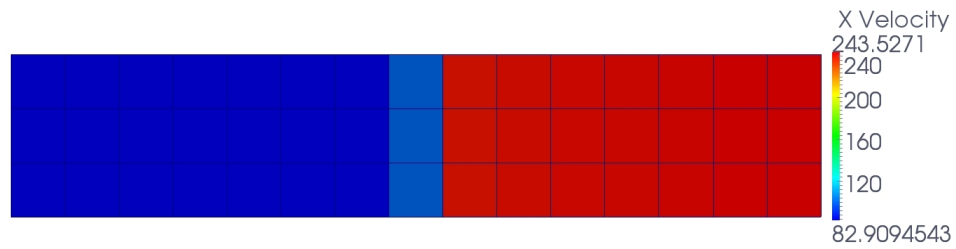
Figure 12: Test case B. Axial velocity distribution around the steady state for mesh 1 in region [0, 5] \times [0, 1] .
