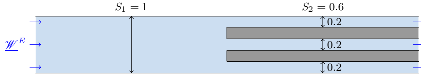
Figure 3: Sketch of test case B. The fluid flows from the left inlet towards the right outlet. On the right hand side, two identical tubes are aligned in the x-direction. The ratio of the right/left flow sections is: S_R/S_L = 3/5 . Inlet values of the density, velocity and pressure are given in section 6.2.
