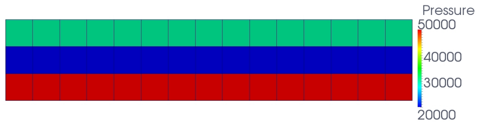
Figure 8: Test case A. Pressure distribution for mesh 2 including 15 \times 3 cells.
