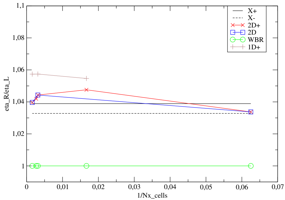
Figure 30: Test case B. Entropy ratio between the right side and the left side of the contraction, as a function of the mesh size h . The blue squares (resp. red crosses) refer to the full two-dimensional simulation (respectively to the new 2D+ approach). Computational results are also compared with those provided by the one-dimensional approach, following either the classical porous (or variable cross section) approach, while using the Well-balanced scheme of Kröner and Thanh (green circles), or the integral 1D+ approach introduced in reference [1] (brown crosses).
