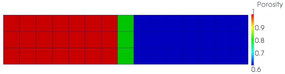
Figure 10: Test case B. Porosity distribution for mesh 1 in region [0, 5] \times [0, 1] .
