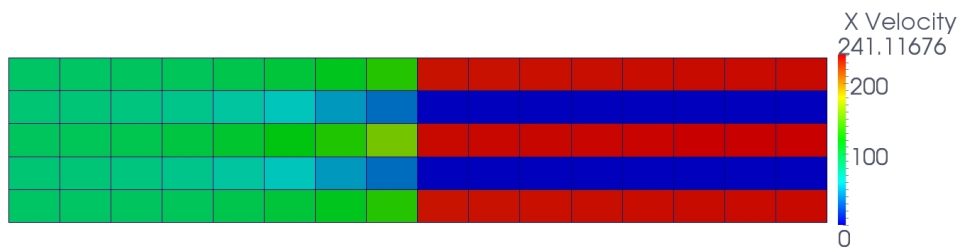
Figure 17: Test case B. Axial velocity distribution around the steady state for mesh 2 in region [0, 5] \times [0, 1] .
