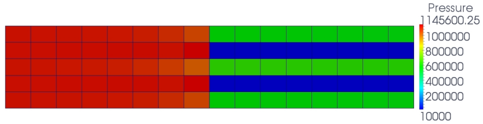
Figure 19: Test case B. Pressure distribution around the steady state for mesh 2 in region [0, 5] \times [0, 1] .
