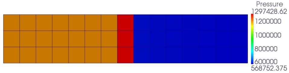
Figure 14: Test case B. Pressure distribution around the steady state for mesh 1 in region [0, 5] \times [0, 1] .
