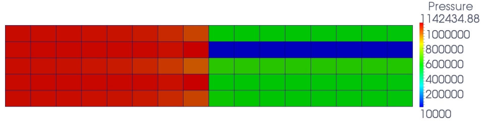
Figure 22: Test case B. Pressure distribution around the steady state for mesh 3 in region [0, 5] \times [0, 1] .
