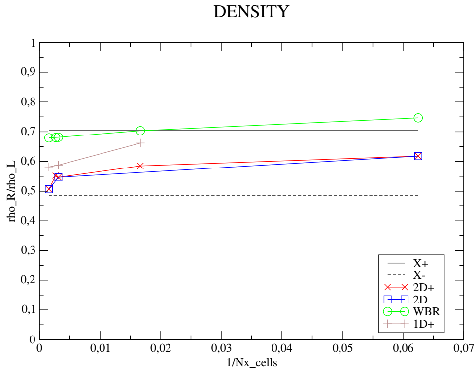
Figure 27: Test case B. Density ratio between the right side and the left side of the contraction, as a function of the mesh size h . The blue squares (resp. red crosses) refer to the full two-dimensional simulation (respectively to the new 2D+ approach). Computational results are also compared with those provided by the one-dimensional approach, following either the classical porous (or variable cross section) approach, while using the Well-balanced scheme of Kröner and Thanh (green circles), or the integral 1D+ approach introduced in reference [1] (brown crosses).
