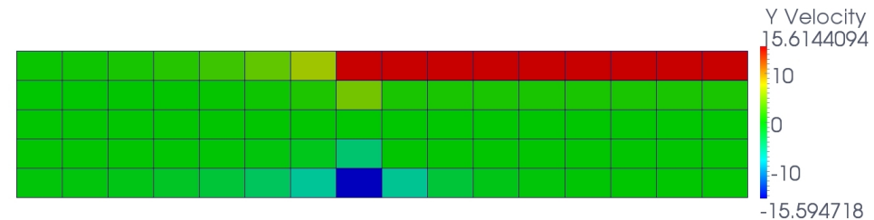
Figure 21: Test case B. Transverse velocity distribution around the steady state for mesh 3 in region [0, 5] \times [0, 1] .
