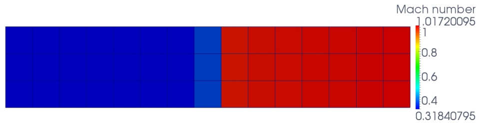
Figure 11: Test case B. Mach number distribution around the steady state for mesh 1 in region [0, 5] \times [0, 1] .
