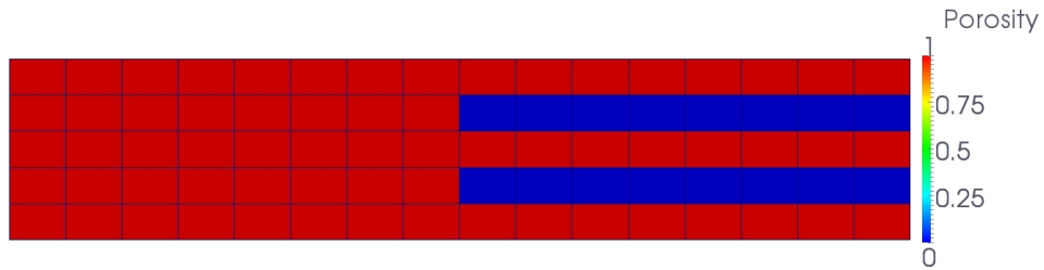
Figure 15: Test case B. Porosity distribution for mesh 2 in region [0, 5] \times [0, 1] .
