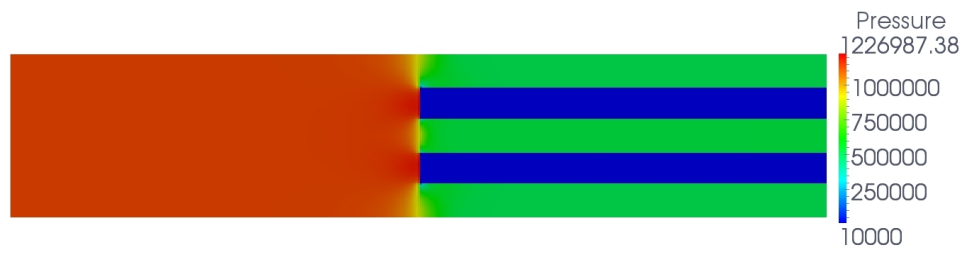
Figure 26: Test case B. Pressure distribution around the steady state for mesh 5 in region [0, 5] \times [0, 1] .
