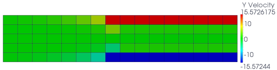
Figure 20: Test case B. Transverse velocity distribution around the steady state for mesh 2 in region [0, 5] \times [0, 1] .
