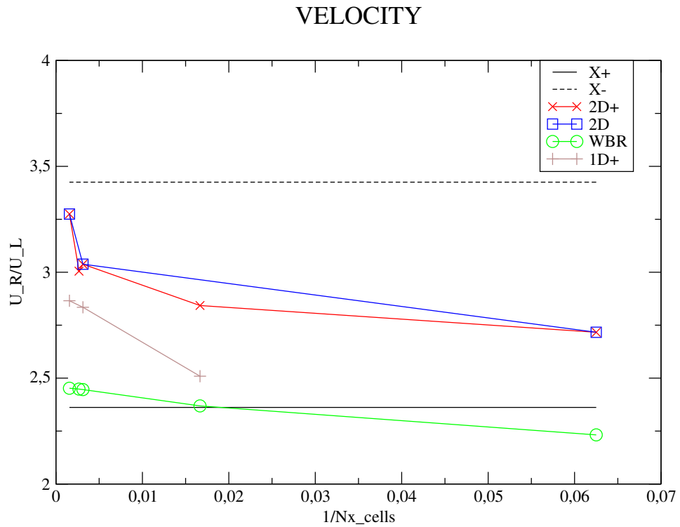
Figure 28: Test case B. Velocity ratio between the right side and the left side of the contraction, as a function of the mesh size h . The blue squares (resp. red crosses) refer to the full two-dimensional simulation (respectively to the new 2D+ approach). Computational results are also compared with those provided by the one-dimensional approach, following either the classical porous (or variable cross section) approach, while using the Well-balanced scheme of Kröner and Thanh (green circles), or the integral 1D+ approach introduced in reference [1] (brown crosses).
