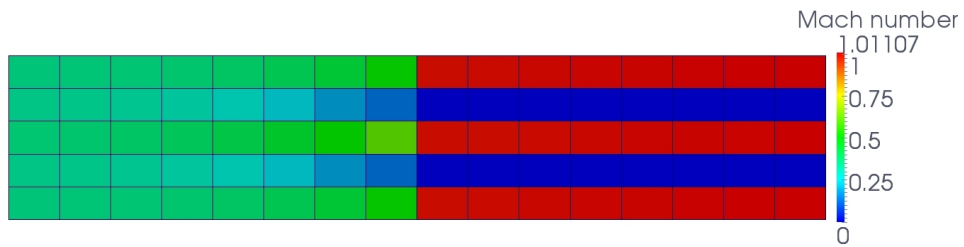
Figure 16: Test case B. Mach number distribution around the steady state for mesh 2 in region [0, 5] \times [0, 1] .
