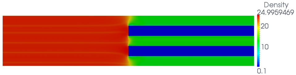
Figure 23: Test case B. Density distribution around the steady state for mesh 4 in region [0, 5] \times [0, 1] .
