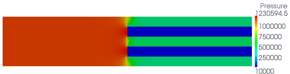
Figure 25: Test case B. Pressure distribution around the steady state for mesh 4 in region [0, 5] \times [0, 1] .
