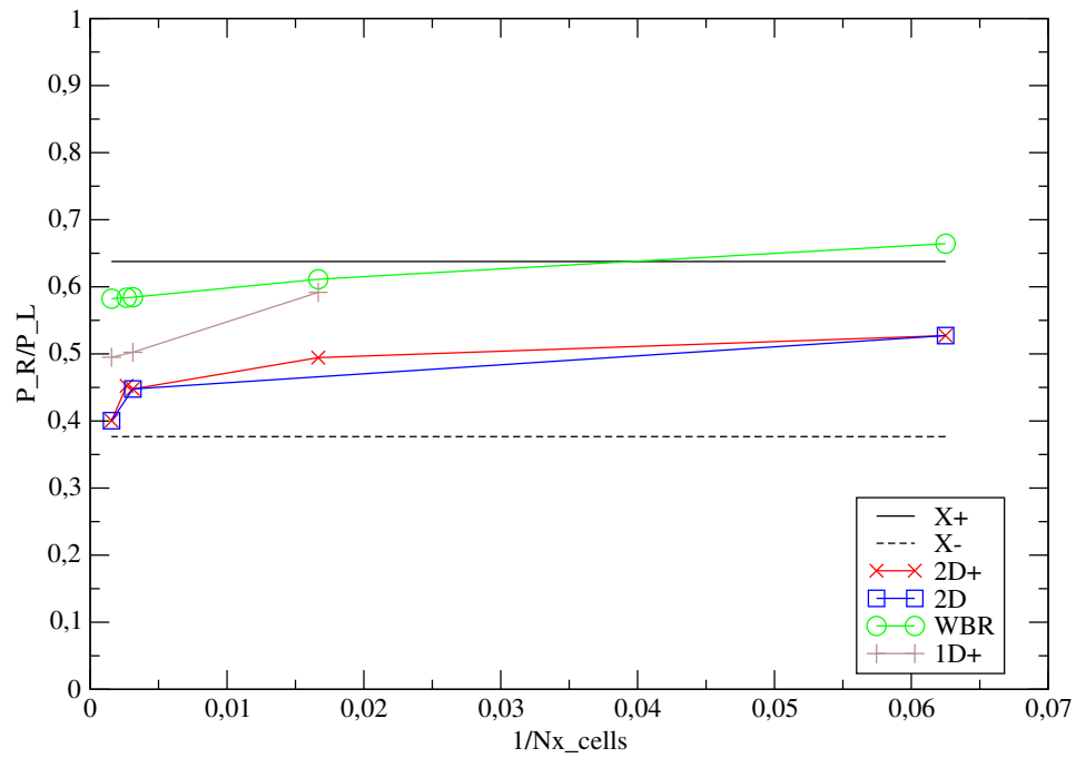
Figure 29: Test case B. Pressure ratio between the right side and the left side of the contraction, as a function of the mesh size h . The blue squares (resp. red crosses) refer to the full two-dimensional simulation (respectively to the new 2D+ approach). Computational results are also compared with those provided by the one-dimensional approach, following either the classical porous (or variable cross section) approach, while using the Well-balanced scheme of Kröner and Thanh (green circles), or the integral 1D+ approach introduced in reference [1] (brown crosses).
