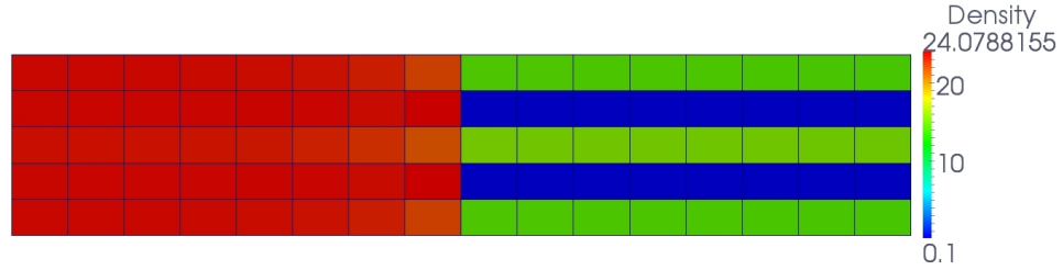
Figure 18: Test case B. Density distribution around the steady state for mesh 2 in region [0, 5] \times [0, 1] .
