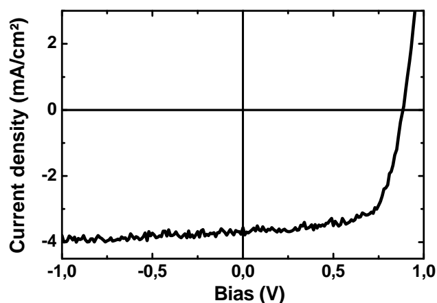
Fig2. Current-voltage measurements under AM1.5G solar spectrum, of a GaP/GaAsPN 300nm/GaP PIN junction grown on a (001)-oriented GaP substrate
