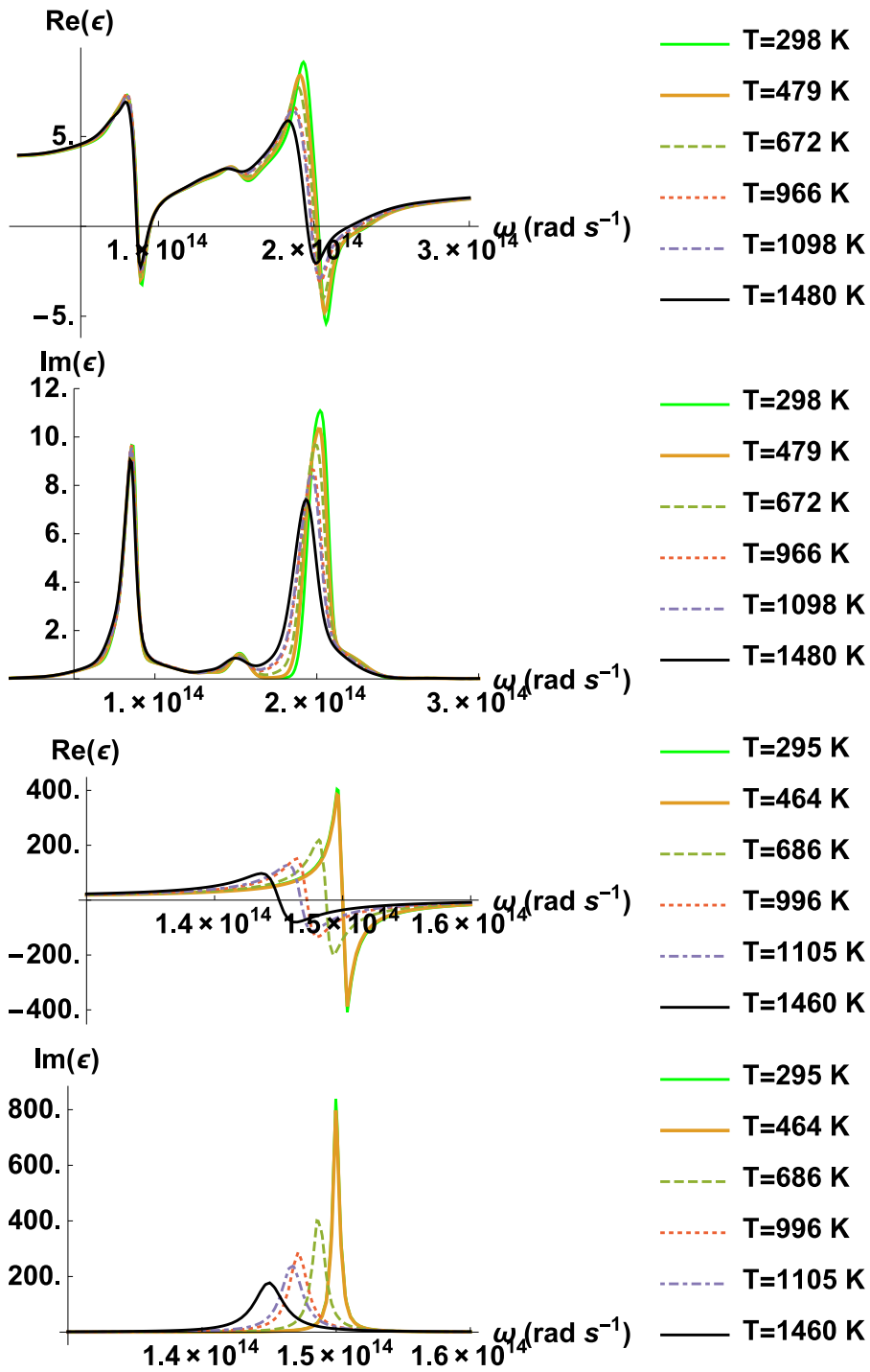
Fig. 1. Measured real and Imaginary part of the dielectric function \epsilon variation with angular frequency \omega for different temperatures. Top 2 figures : SiO 2 . Bottom 2 figures : SiC.
