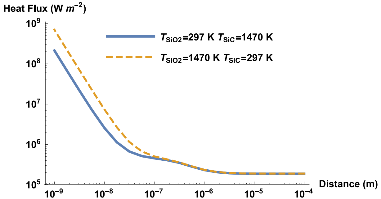
FIG. 2: Radiative heat transfer between a plane interface of SiC and a second one constituted of SiO 2 versus their separation distances. Two situations are compared. In the first one (plain) SiO 2 is at 297 K and SiC at 1470 K whereas in the second one (dashed) SiC is at 297 K and SiO 2 is at 1470 K.
