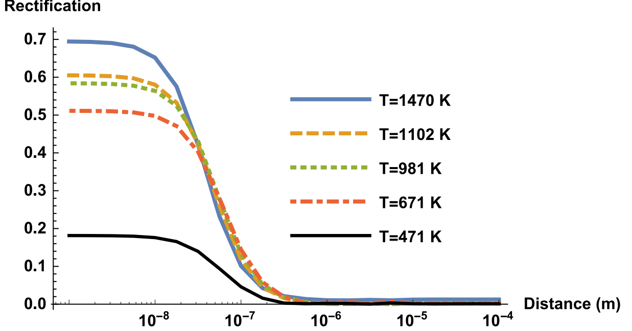
FIG. 3: Rectification variations as a function of the separation distance between two planar interfaces made of SiC and SiO 2 when one material is at 297 K and the second one at 471 K, 671 K, 981 K, 1102 K or 1470 K.
