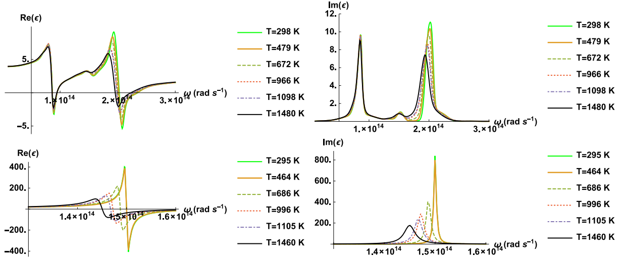
FIG. 1: Real and Imaginary part of the dielectric function \epsilon variation with angular frequency \omega for different temperatures. Top : \text{SiO}_2 . Bottom \text{SiC} .
