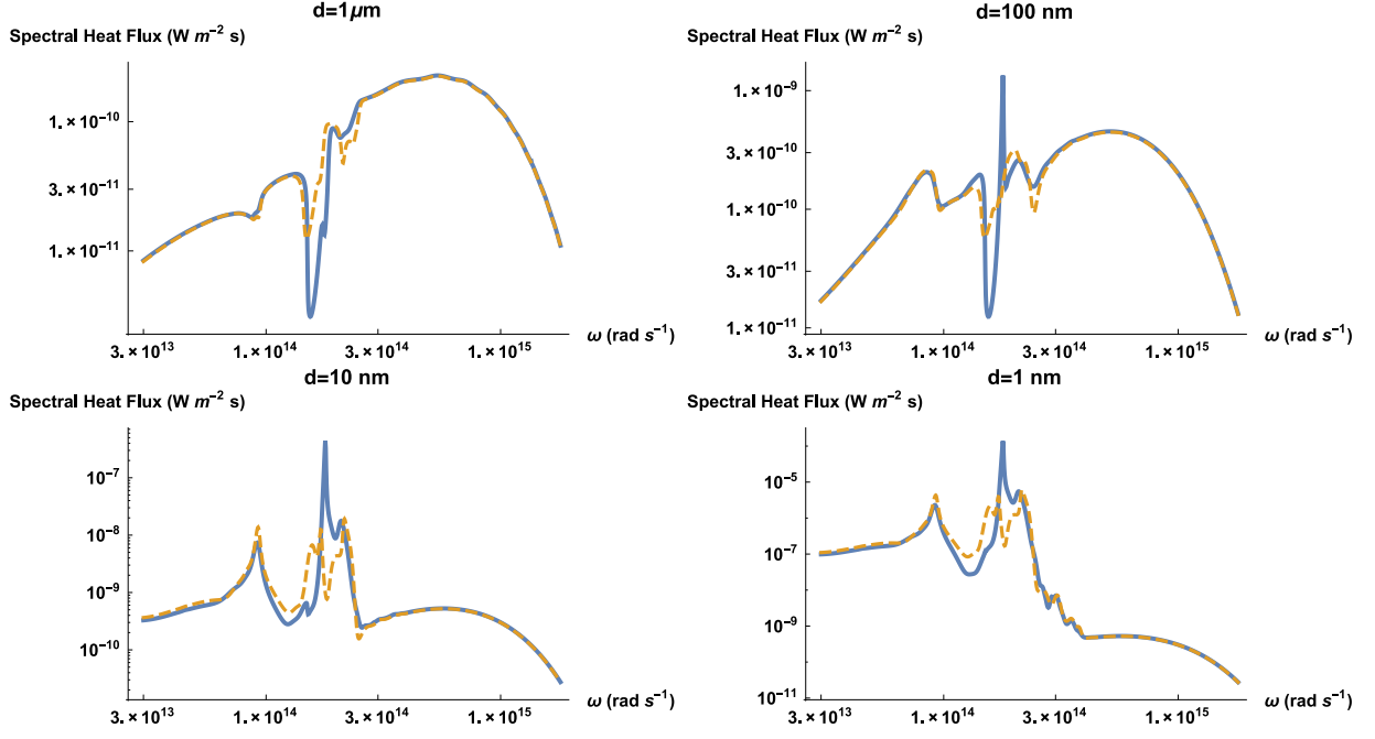
FIG. 4: Spectral radiative heat transfer between two planar interfaces made of SiC and SiO 2 in the direct and the reverse situation : SiO 2 is at 297 K and SiC is at 1470 K in the first situation (plain) whereas SiO 2 is at 1470 K and SiC is at 297 K in the second situation (dashed).
