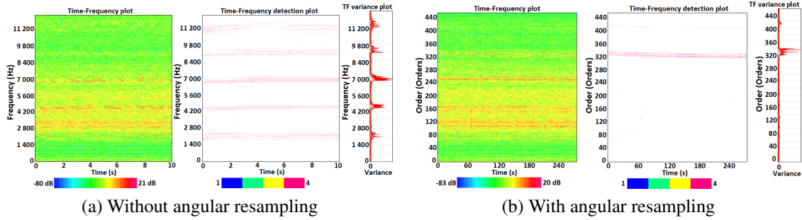
Figure 8: The spectrogram and the non-stationarity detection results of the same signal ( 75^{th} measurement) without (a) and with (b) the angular resampling (sampled at 911.7 orders). The time-frequency spectrogram (left), non-stationarity detection (middle) and its variance (right).
