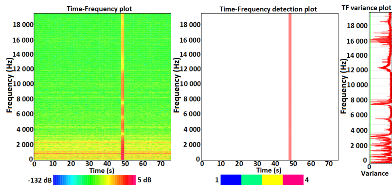
Figure 5: Time-frequency spectrogram (left), non-stationarity detection (middle) and its variance (right) of the signal at operating time of 168.57 hours.
