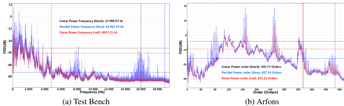
Figure 3: Power spectral density (PSD) of the signal acquired from (a) Test bench data at operating time of 85.97 hours. (b) Arfons data of the 77 th signal.
