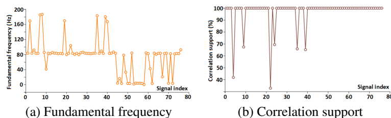
Figure 11: Surveillance of the periodicity tests on 77 signals of accelerometer A6. (a) Detected fundamental frequency (b) Correlation support.
