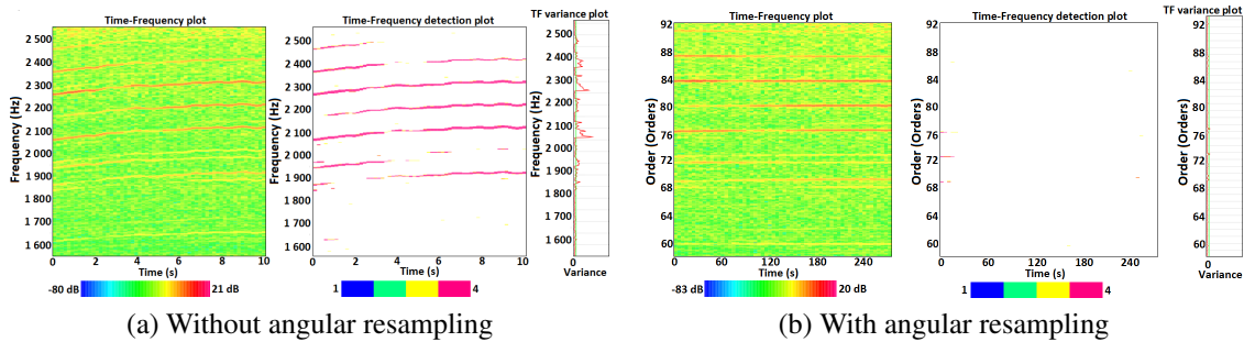
Figure 9: A zoomed presentation of the results of Fig. 8 at the medium and the low frequency range (lower than 2500 Hz and lower than 92 orders)
