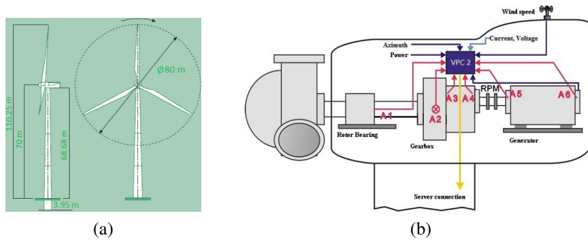
Figure 7: General information of the wind turbines under study. (a) Dimensions of the wind turbines. (b) Location of the installed sensors.
