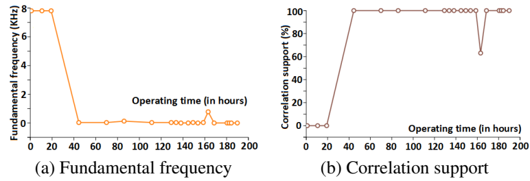
Figure 6: Surveillance of the periodicity tests of accelerometer (+y) (main bearing of the test bench) from 0,96 hours to 189.85 hours of operation. (a) Detected fundamental frequency (b) Correlation support of the signal length.
