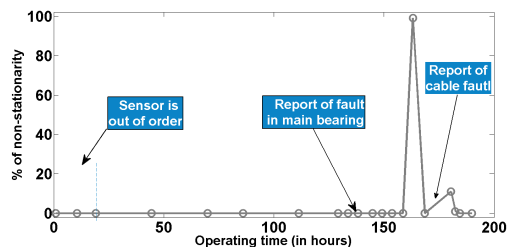
Figure 4: Surveillance of the non-stationarity test of accelerometer (+y) (main bearing of the test bench) from 0.96 hours to 189.85 hours of operation.
