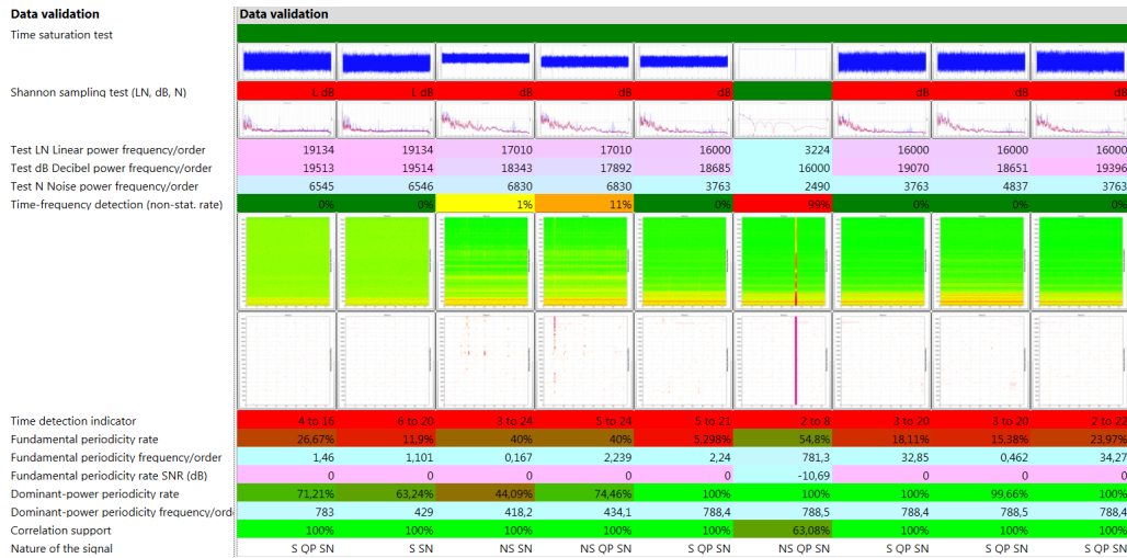
Figure 2: The behaviour of AStrion-D over time. Green colour is OK, red colour is ALARM. S is for stationary, QP quasi-periodic and SN significant noise.
