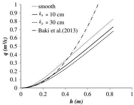
Fig. 20. Influence of bed roughness in a full-scale fishpass (slope = 5%, D = 50 \text{ cm} , C = 13\% )
