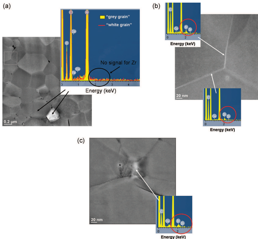
Fig. 4. HAADF observations and EDX measurements of AZ570 sample sintered at T_f = 1300^\circ\text{C} (a) global view, (b) zoom of the grain boundaries, and (c) secondary phase particle observation. Bright contrasts on grain boundaries correspond to \text{Zr}^{4+} segregation. Arrows indicate the EDX analysis point.
