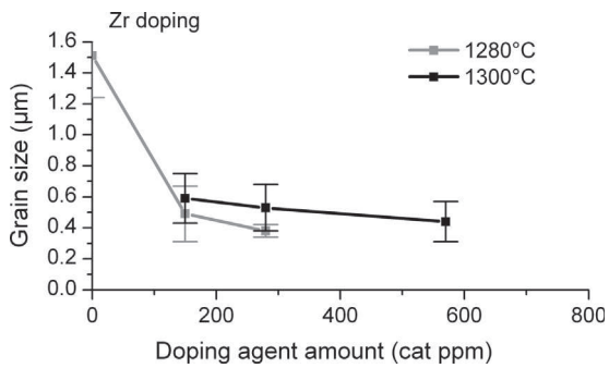
Fig. 3. Average grain sizes of Zr-doped alumina samples sintered at T_f = 1280^\circ\text{C} and 1300^\circ\text{C} for different amounts of doping agent.
