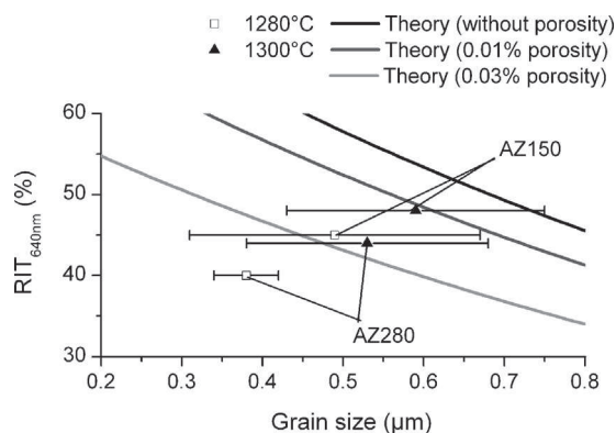
Fig. 6. Comparison of RIT s640nm of AZ150 and AZ280 samples sintered at T_f = 1280^\circ\text{C} and 1300^\circ\text{C} with theoretical models ( \lambda_0 = 640\text{ nm} , D = 0.88\text{ }\mu\text{m} , \phi_p = 100\text{ nm} ).
