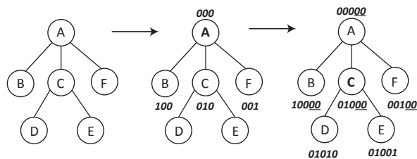
Figure 1: Construction of isometric embedding on a sample tree. For this six nodes tree, the embedding requires five bits.
