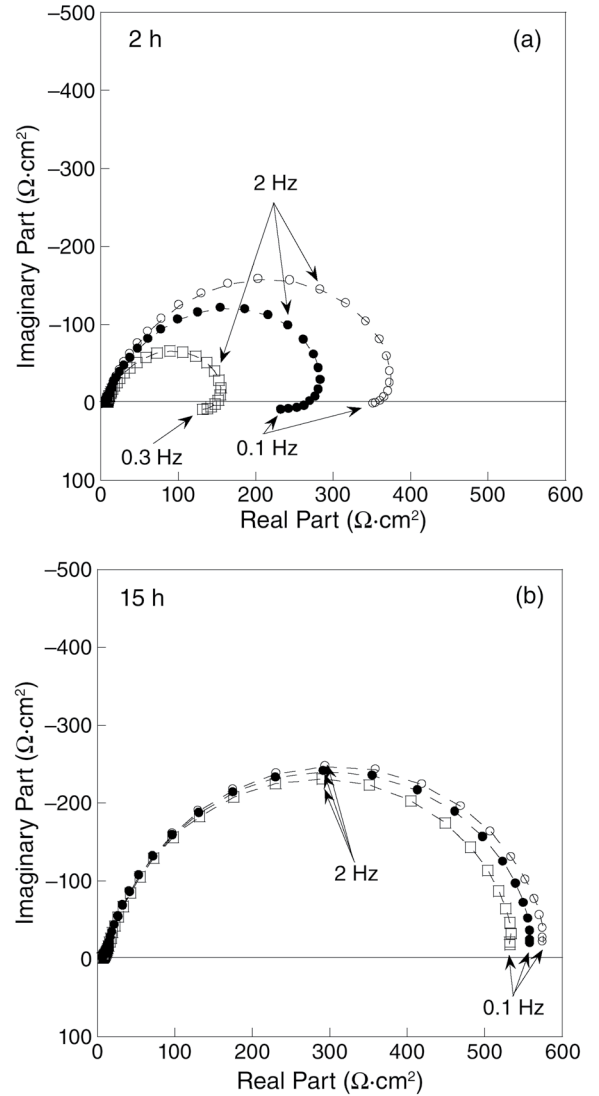
FIGURE 6. Electrochemical impedance diagrams plotted consecutively at the corrosion potential after (a) 2 h and (b) 15 h of immersion in a 0.5 M NaCl solution saturated with CO_2 : (○) 400 rpm, (●) 1,000 rpm, and (□) 1,600 rpm.
