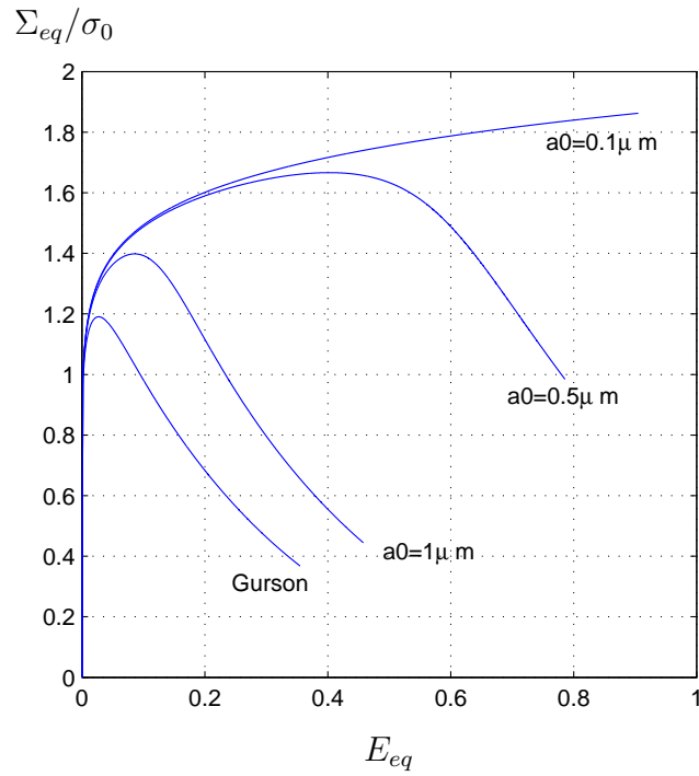
Fig. 6. Normalized equivalent stress vs the effective strain for various values the initial cavity size and the Gurson model. Case of a triaxiality T = 3 .
