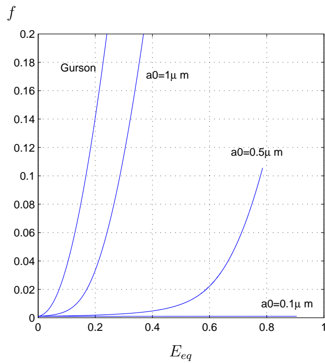
Fig. 7. Porosity vs the effective strain for various values the initial cavity size and the Gurson model. Case of a triaxiality T = 3 .
