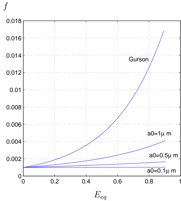
Fig. 5. Porosity vs the effective strain for various values the initial cavity size and the Gurson model. Case of a triaxiality T = 1 .
