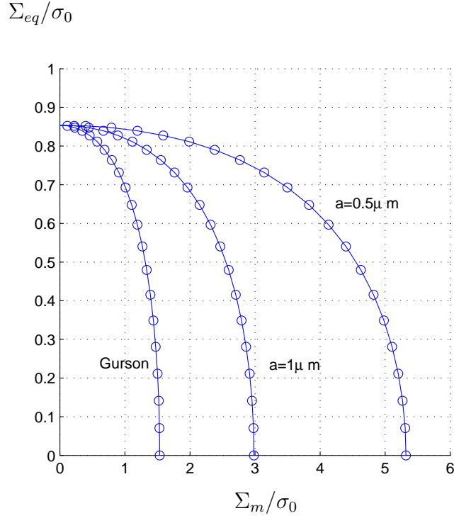
Fig. 3. Macroscopic yield surface for the porosity f = 0.1 and for a_0 = 0.5\mu m , a_0 = 1\mu m and a_0 \gg l_{SG} (Gurson).
