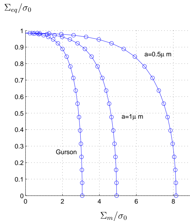
Fig. 2. Macroscopic yield surface for the porosity f = 0.01 and for a_0 = 0.5\mu m , a_0 = 1\mu m and a_0 \gg l_{SG} (Gurson).
