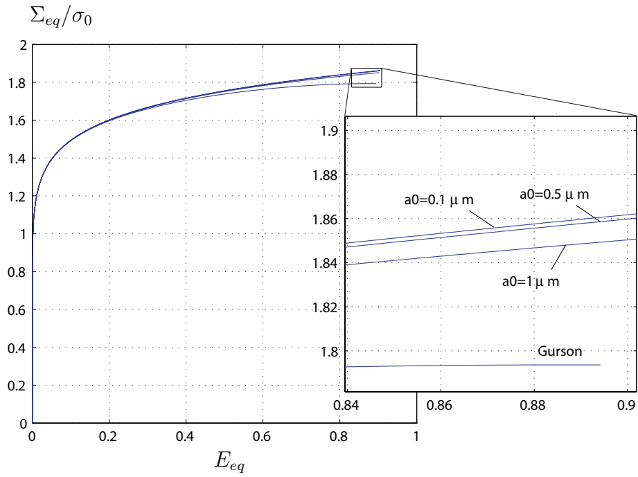
Fig. 4. Normalized equivalent stress vs the effective strain for various values the initial cavity size and the Gurson model. Case of a triaxiality T = 1 .
