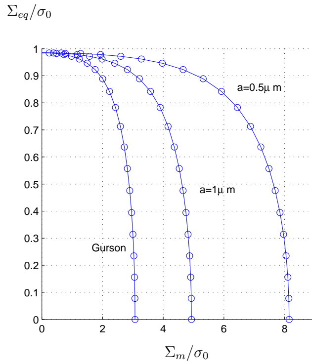
Fig. 2. Macroscopic yield surface for the porosity f = 0.01 and for a_0 = 0.5\mu\text{m} , a_0 = 1\mu\text{m} and a_0 \gg l_{SG} (Gurson).
