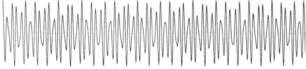
Figure 3. The octagonal density function f_3(x) when the coordinate x lies in the range [0, 100] . Note the large number of peaks at rather regular distances.
