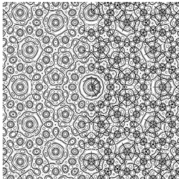
Figure 15. Density levels for n_4(x, y) , x, y \in [-10, 10] , maxima and links for x \in [0, 10] . On line red =+4, pink=+3, orange=+2, black=+1, sky blue=0, dark blue=-1, dark blue=-2. On paper grey levels are seen.
