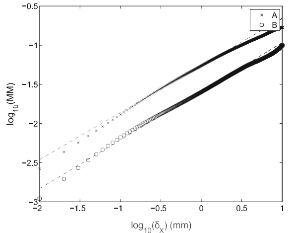
Fig. 7 Statistical data analysis MM obtained by the characterization of fracture surfaces of RT-PMMA (A and B) probed by OMP (sample JBK6); linear fitting for \log(\delta) \in [-2;1] for regimes (A) and (B) with slopes \beta_A = 0.60 and \beta_B = 0.62
