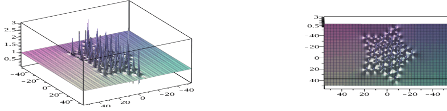
Figure 5: Solution of NLS, N=10 , \tilde{b}_2 = 10^5 : 8 rings without a peak in the center; on the right, sight of top.
