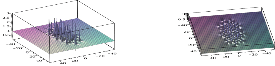
Figure 8: Solution of NLS, N=10 , \tilde{a}_4 = 10^8 : 5 rings with a central peak; on the right, sight of top.
