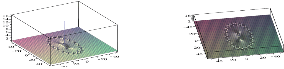
Figure 18: Solution of NLS, N=10 , \tilde{a}_9 = 10^{19} : one ring with in the center the Peregrine breather of order 8; on the right, sight of top.
