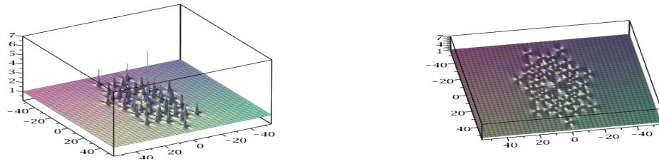
Figure 6: Solution of NLS, N=10 , \tilde{a}_3 = 10^7 : 4 rings with in the center P_3 ; on the right, sight of top.
