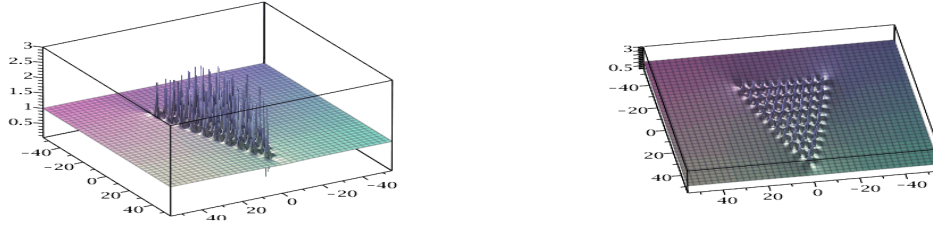
Figure 2: Solution of NLS, N=10 , \tilde{a}_1 = 10^3 : triangle with 55 peaks; on the right, sight of top.
