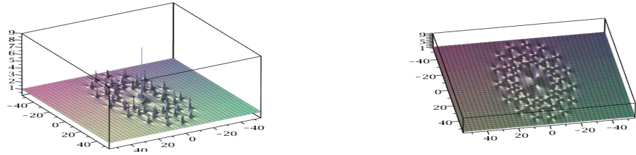
Figure 15: Solution of NLS, N=9 , \tilde{b}_7 = 10^{16} : 3 rings with in the center the Peregrine breather of order 4; on the right, sight of top.
