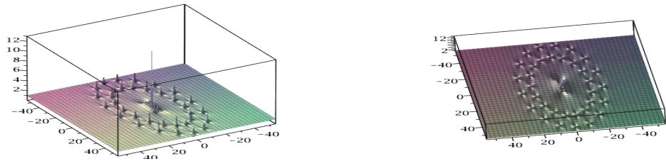
Figure 16: Solution of NLS, N=10 , \tilde{a}_8 = 10^{19} : 2 ring with in the center the Peregrine breather of order 6; on the right, sight of top.
