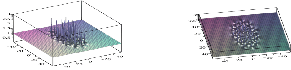
Figure 11: Solution of NLS, N=10 , \tilde{b}_5 = 10^{10} : 5 rings without a central one peak; on the right, sight of top.
