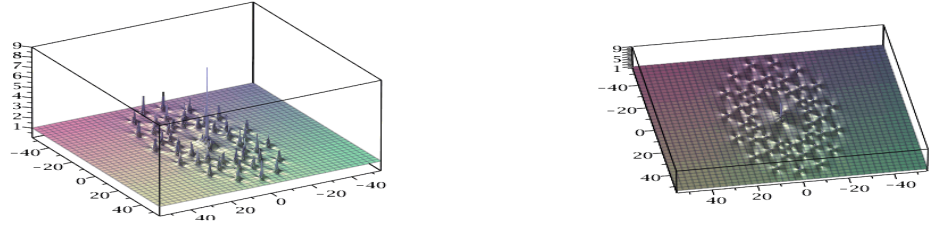
Figure 14: Solution of NLS, N=10 , \tilde{a}_7 = 10^{16} : 3 rings with in the center the Peregrine breather of order 4; on the right, sight of top.
