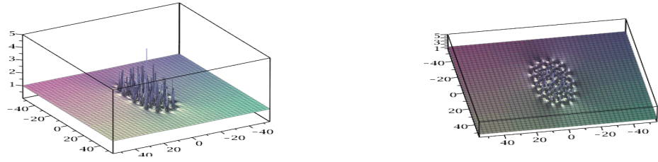
Figure 12: Solution of NLS, N=10 , \tilde{a}_6 = 10^{10} : 4 rings with in the center the Peregrine breather of order 2; on the right, sight of top.
