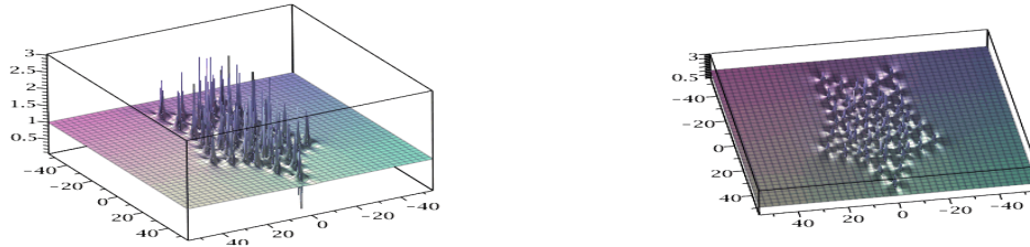
Figure 4: Solution of NLS, N=10 , \tilde{a}_2 = 10^5 : 8 rings without a peak in the center; on the right, sight of top.
