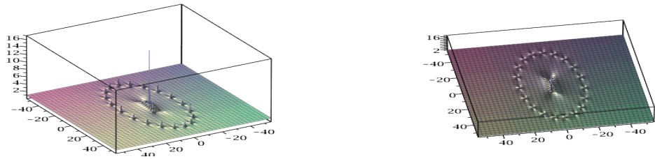
Figure 19: Solution of NLS, N=10 , \tilde{b}_9 = 10^{19} : one ring with in the center the Peregrine breather of order 8; on the right, sight of top.
