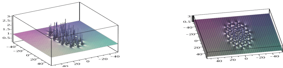
Figure 10: Solution of NLS, N=10 , \tilde{a}_5 = 10^{10} : 5 rings without a central one peak; on the right, sight of top.
