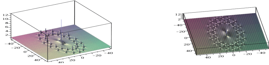
Figure 17: Solution of NLS, N=10 , \tilde{b}_8 = 10^{19} : 2 ring with in the center the Peregrine breather of order 6; on the right, sight of top.
