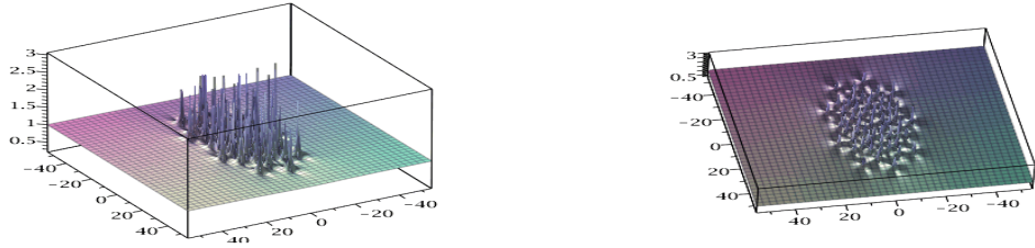
Figure 9: Solution of NLS, N=10 , \tilde{b}_4 = 10^8 : 5 rings with a central peak; on the right, sight of top.
