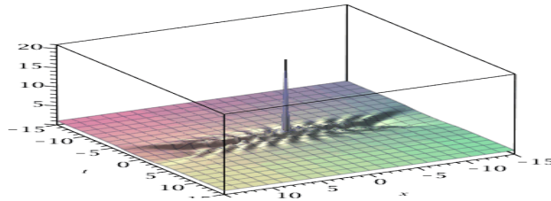
Figure 1: Solution of NLS, N=10, all parameters equal to 0, Peregrine breather P_{10} .
