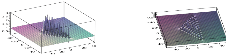
Figure 3: Solution of NLS, N=10 , \tilde{b}_1 = 10^3 : triangle with 55 peaks; on the right, sight of top.
