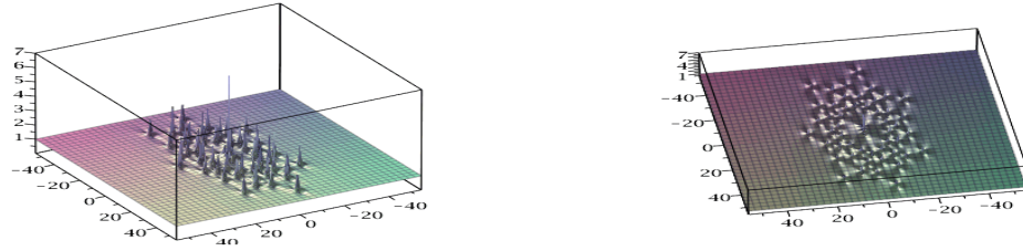
Figure 7: Solution of NLS, N=10 , \tilde{b}_3 = 10^7 : 4 rings with in the center P_3 ; on the right, sight of top.
