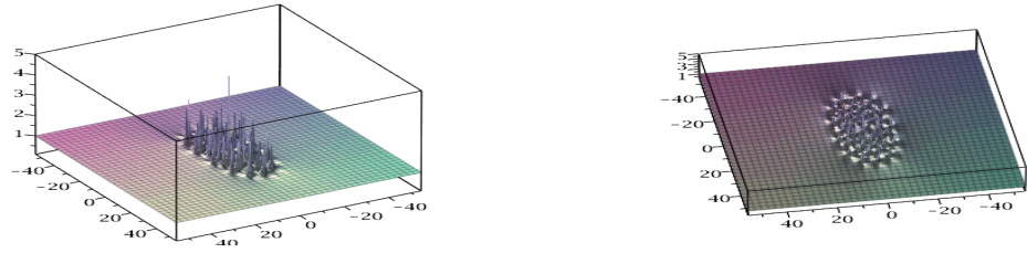
Figure 13: Solution of NLS, N=10 , \tilde{b}_6 = 10^{10} : 4 rings with in the center the Peregrine breather of order 2; on the right, sight of top.
