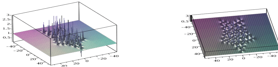
Figure 4: Solution of NLS, N=10 , \tilde{a}_2 = 10^5 : 8 rings without a peak in the center; on the right, sight of top.
