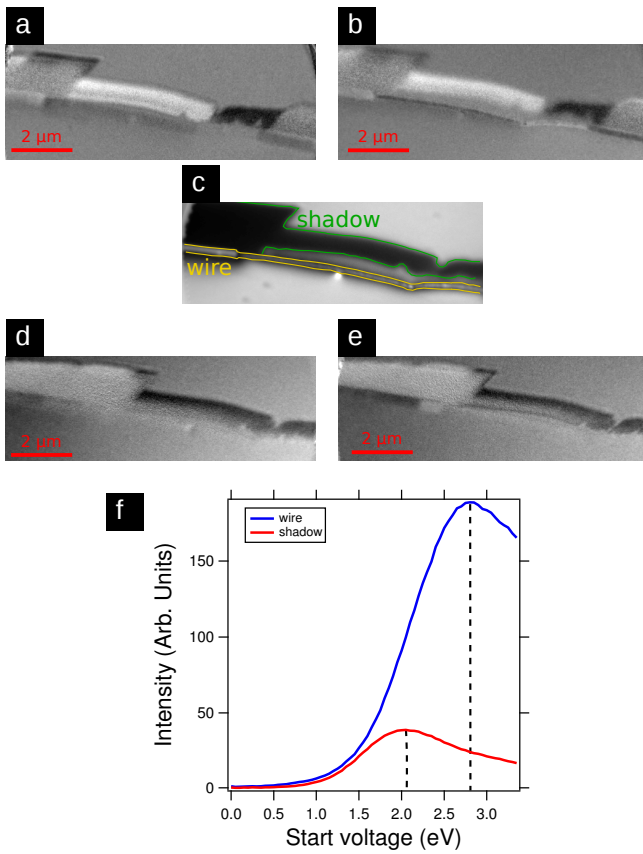
Figure 7: Role of the plane of focus and the start voltage) The XMCD contrast is taken at the Fe L3 edge, with start voltage 2.1 eV with a focus (a) on the surface and (b) on the wire. (c) is the sum of both helicity intensities where the wire and shadow areas are highlighted to guide the eye. (d) 2.0 eV and (e) 2.8 eV with a focus on the surface. (f) XAS on the wire and the shadow versus the start voltage.
