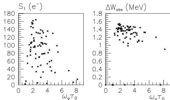
FIG. 2. Variations of S_1 (left) and of \Delta W_{\text{obs}} (right) with \omega_p \tau_0 . The fitting procedure ( S_1 > 10e^- ) introduces a cutoff at \Delta W_{\text{obs}} = 0.85 \text{ MeV} . The pressure is varied in the range 0–2 mbar with half of the data taken at “resonance.” The main source of variation of \omega_p \tau_0 is the fluctuation of \tau_0 . Only data with \tau < 1 \text{ ps} are used.
