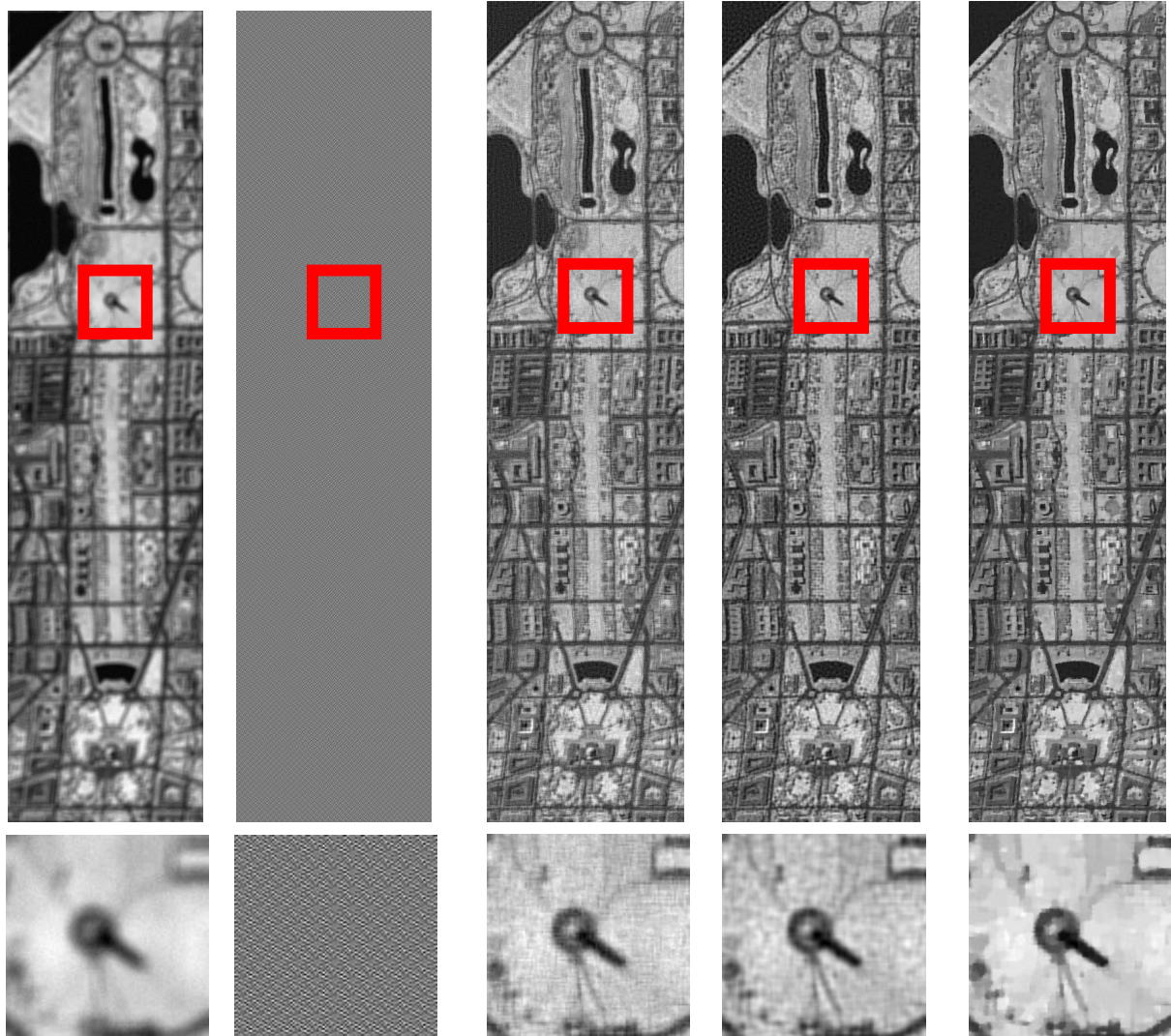
(a) Degraded Uniform blur 9 \times 9 Gaussian noise (b) Inverse filtering (c) Quadratic regularisation \Lambda = \text{Id} (d) \Lambda Laplacian (e) Total variation regularization
