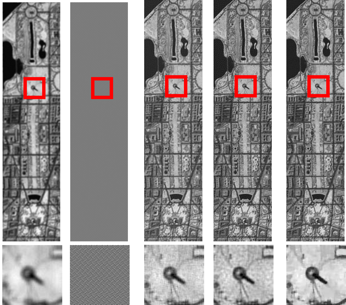
(a) Degraded Uniform blur 9 \times 9 Gaussian noise (b) Inverse filtering (c) Quadratic regularisation \Lambda = \text{Id} (d) \Lambda Laplacian (e) Total variation regularization
