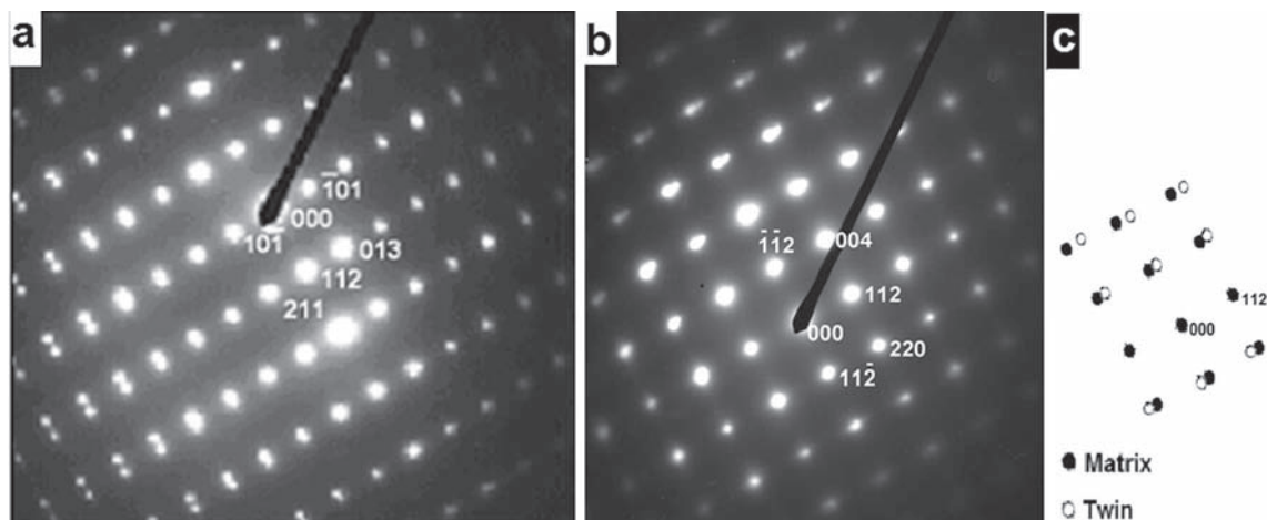
Fig. 8. Selected area electron diffraction (SAED) patterns of a single quadratic phase \text{Mn}_{3-x}\text{Co}_x\text{O}_4 ceramic sample for x = 1.54 : (a) along the zone axis [1\bar{1}0] , (b) along the zone axis [1\bar{1}0] , and (c) schematic reproduction of a part of (b). These patterns exhibit splitting of spots (in such a way that there are spots corresponding to the matrix and other spots corresponding to twins which are deduced from the first ones by reflection from a plane mirror coinciding with the twin interface plane). The reflections that are not split correspond to crystallographic rows perpendicular to the (1 1 2) twin interface plane. The magnitude of splitting increases with the distance from the center of the pattern.
